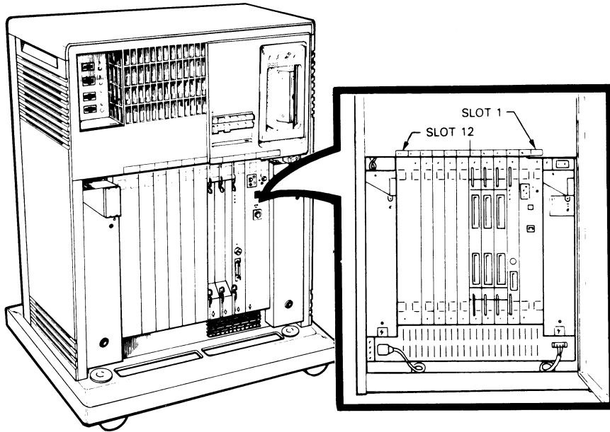
Figure 1–10: Card Cage
