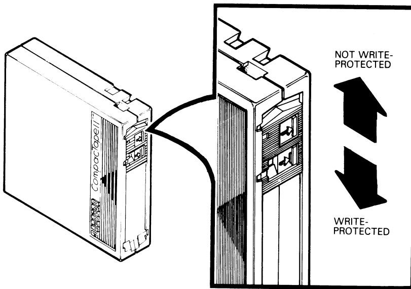
Figure 3-5: Tape Cartridge Write-Protect Switch
