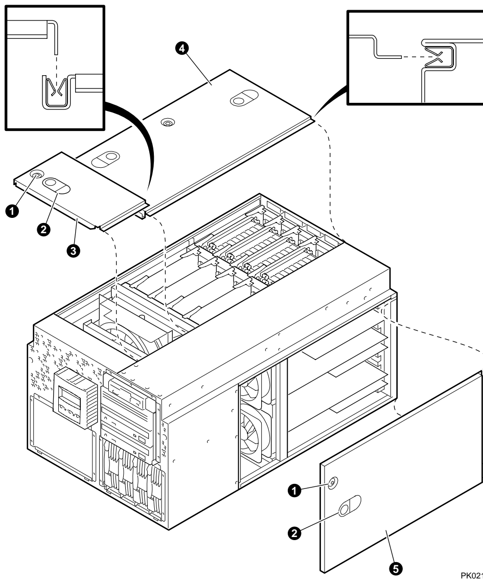
Figure 2-6 Removing Covers from a Pedestal/Rack
