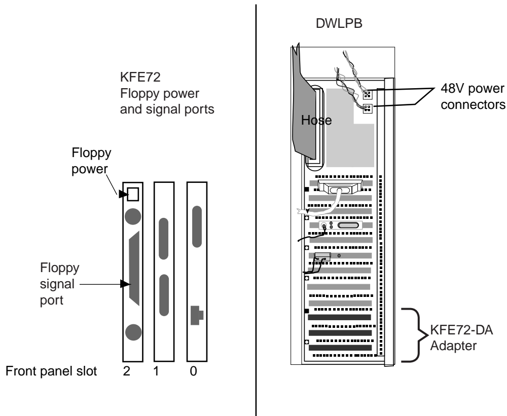
Figure 2-11 Relevant Connectors on KFE72s and DWLPBs
