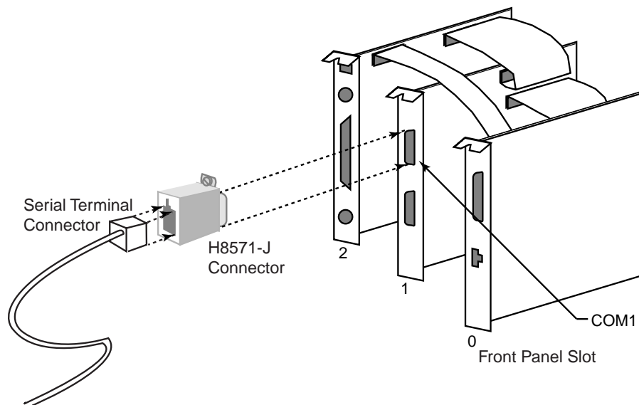
Figure 2-8 KFE72-DA Adapters
