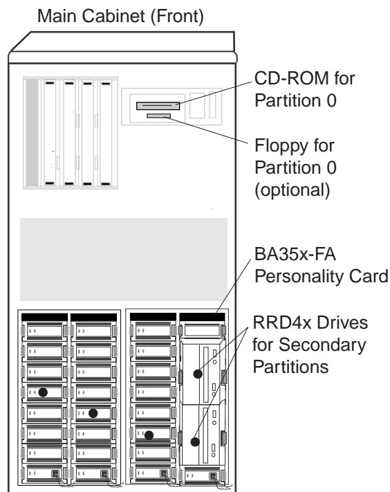
Figure 2-9 Placement of RRD4x-VA Drives
