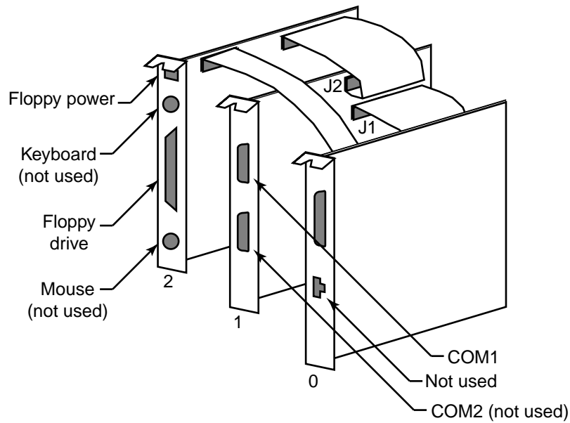
Figure 2-10 Floppy Drive Connector on KFE72-DA Adapter
