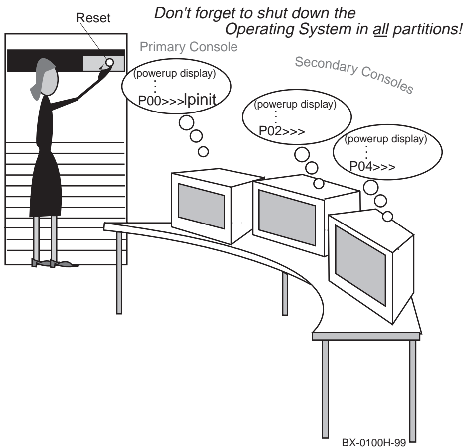
Figure 5-1 Setting auto_action to Halt in Each Partition
