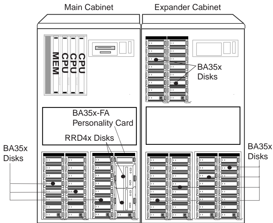
Figure 2-1 Sample Configuration (Front View of Cabs)
