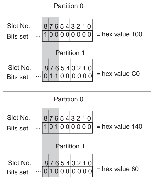
Figure 3-5 Construction of Two-Partition I/O Bit Masks
