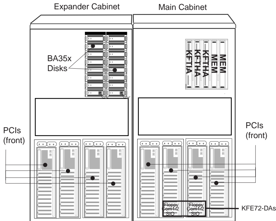
Figure 2-2 Sample Configuration (Rear View of Cabs)
