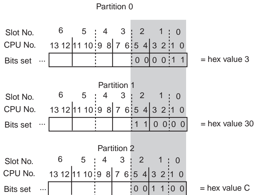
Figure 3-2 Construction of Three-Partition CPU Bit Mask
