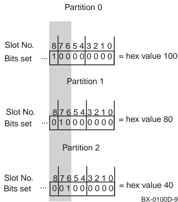
Figure 3-4 Construction of Three-Partition I/O Bit Masks
