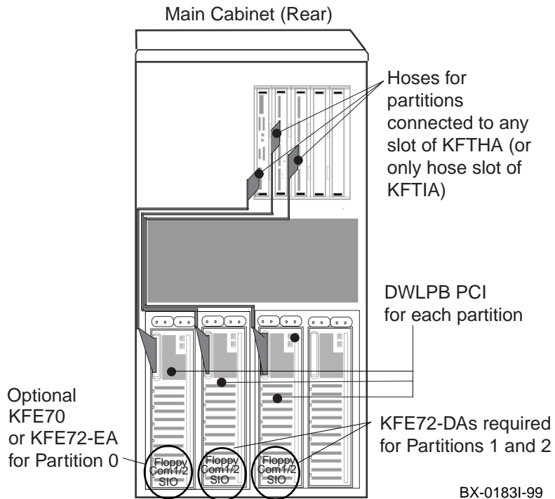
Figure 2-6 DWLPB PCI Card Cages
