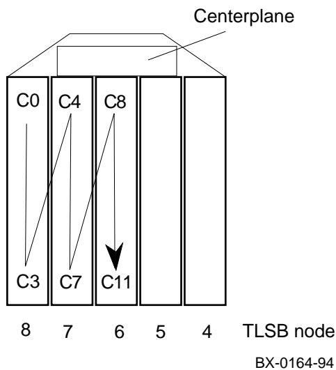
Figure 2-7 Hose Numbering Scheme for I/O Modules
