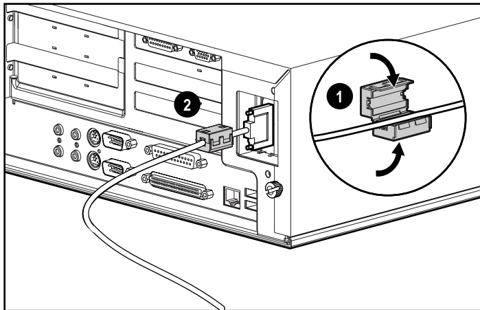
Figure 1: Attaching the Ferrite Bead
