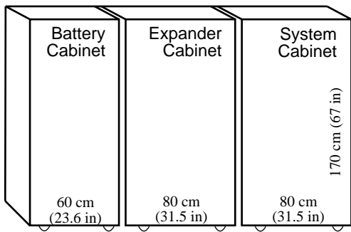
Figure 1-4 Three-Cabinet System (Front Dimensions)
