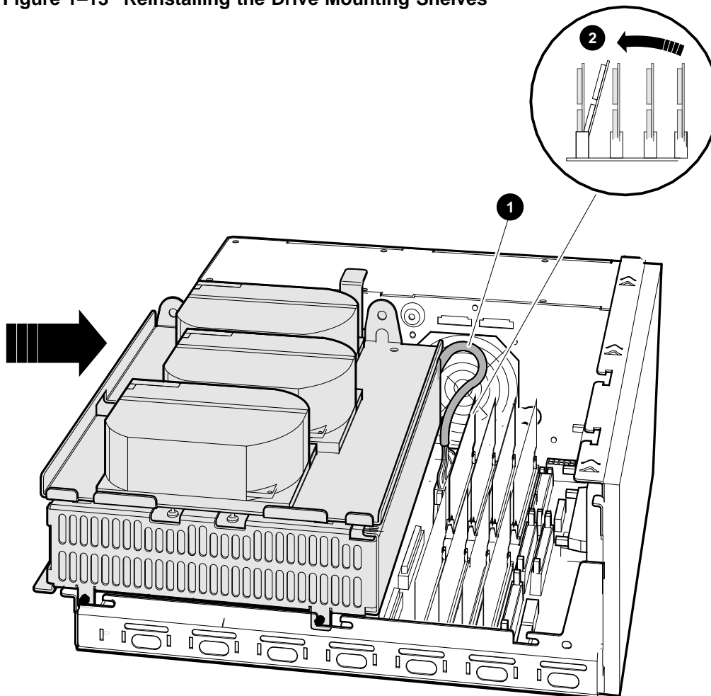
Figure 1–13 Reinstalling the Drive Mounting Shelves
