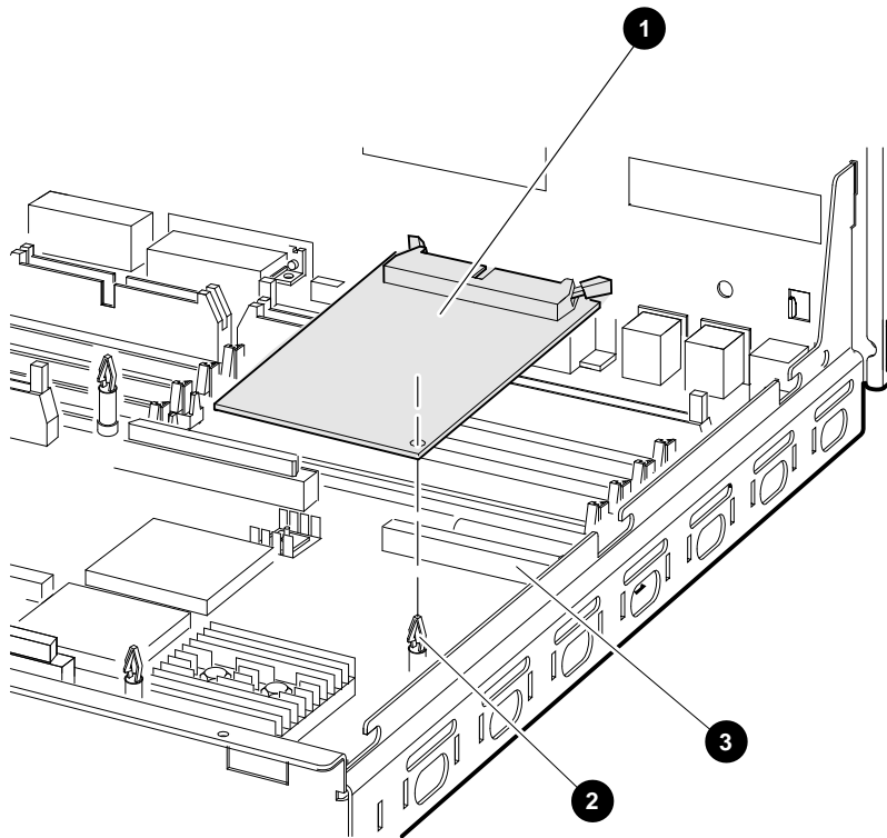
Figure 1–10 Installing the SCSI Daughter Card
