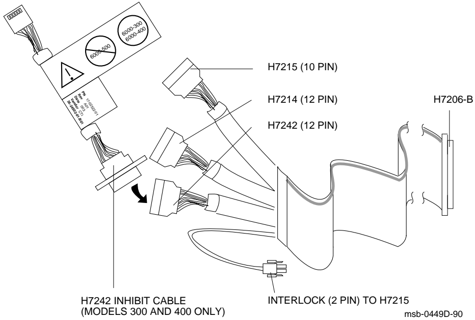
Figure 2-4: Control/Status Cable
