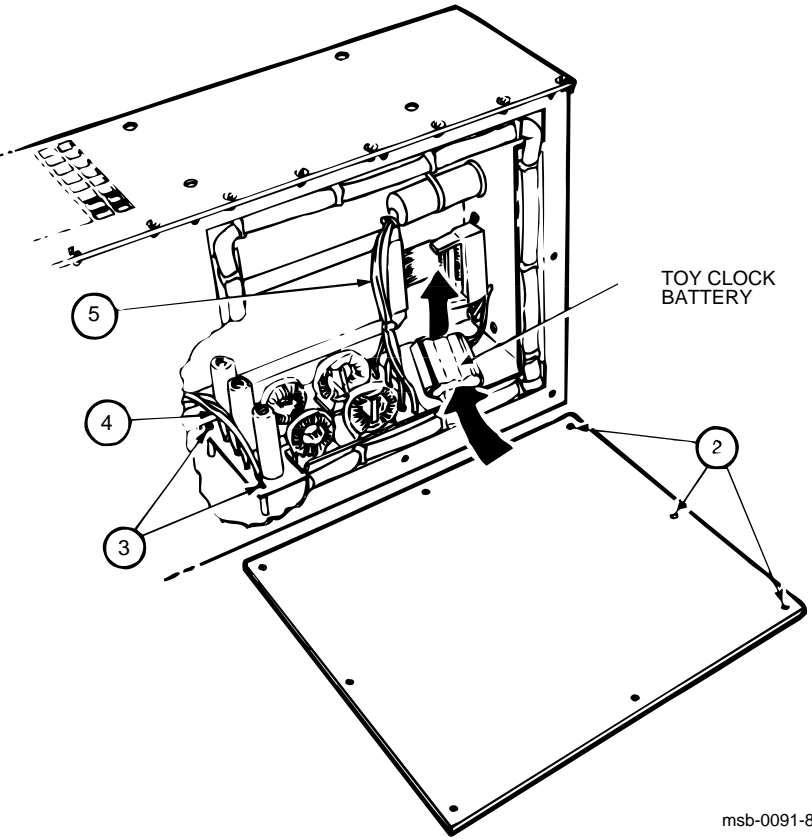
Figure 4-9: Filter Board and TOY Clock Battery Removal
