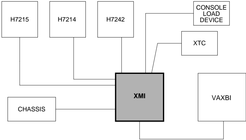
Figure 2-1: XMI Card Cage Connections
