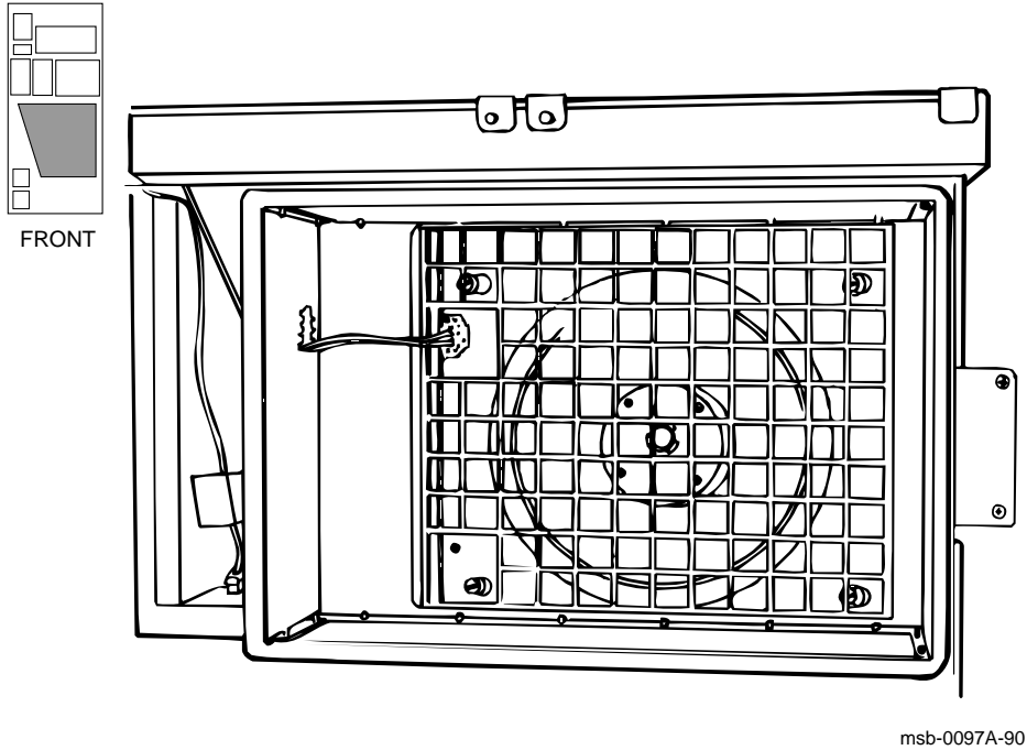
Figure 6-6: Front Blower
