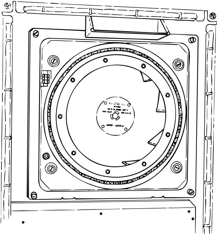
Figure 6-5: Blower Assembly
