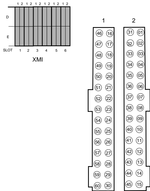
Figure B-1: XMI Backplane Connector Numbering
