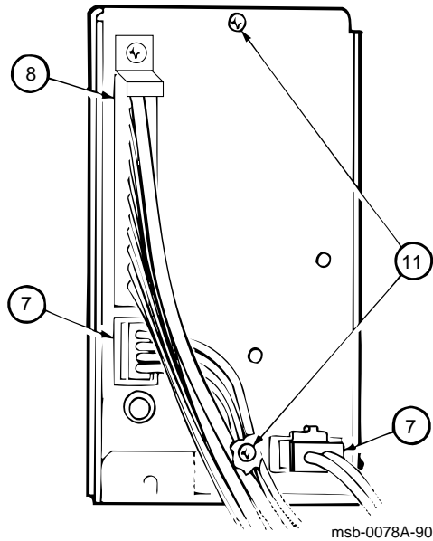
Figure 5-7: H7215 Power Regulator Removal
