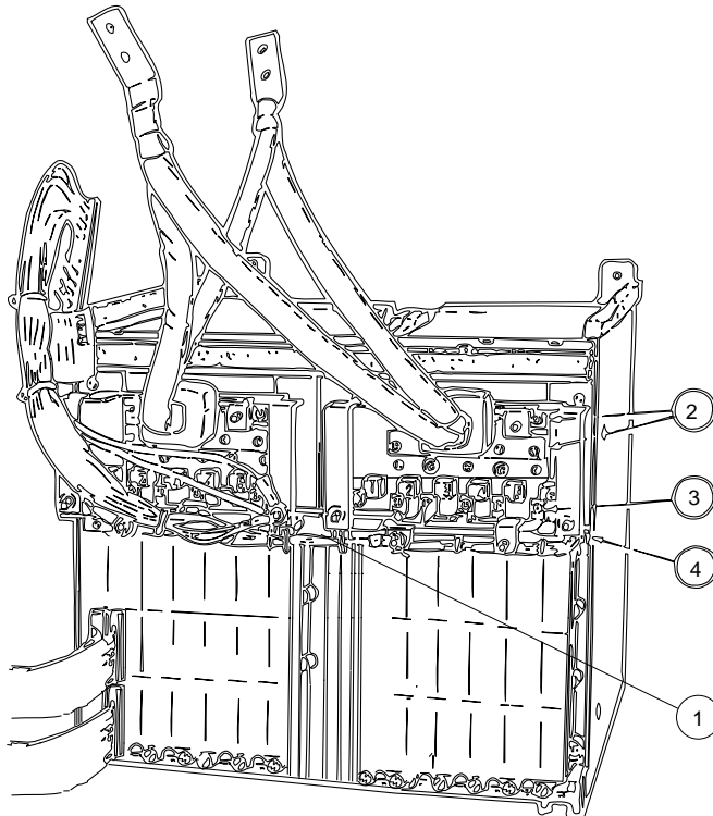
Figure 3-6: VAXBI Bus Bar Assembly
