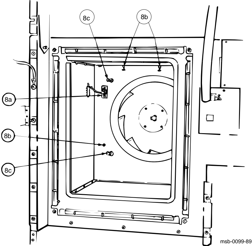
Figure 6-8: Blower Assembly Removal (Rear View)
