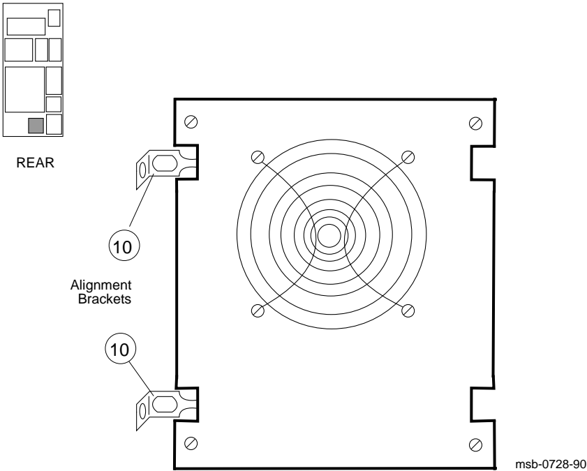
Figure 5-23: H7236-A BBU Enclosure Removal
