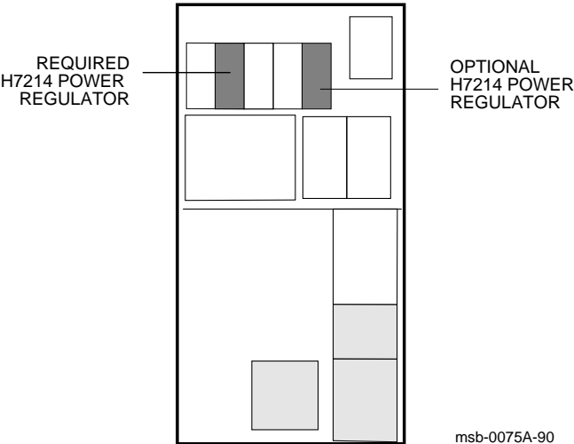
Figure 5-4: H7214 Power Regulators (Rear View)
