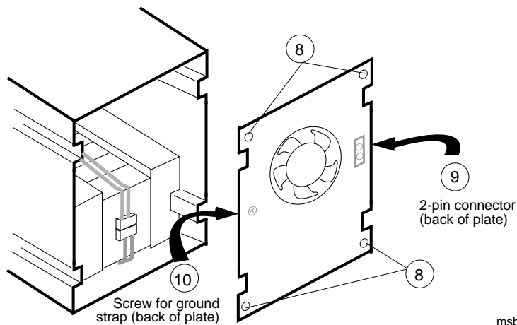
Figure 5–20: H7236-A BBU Fan Removal
