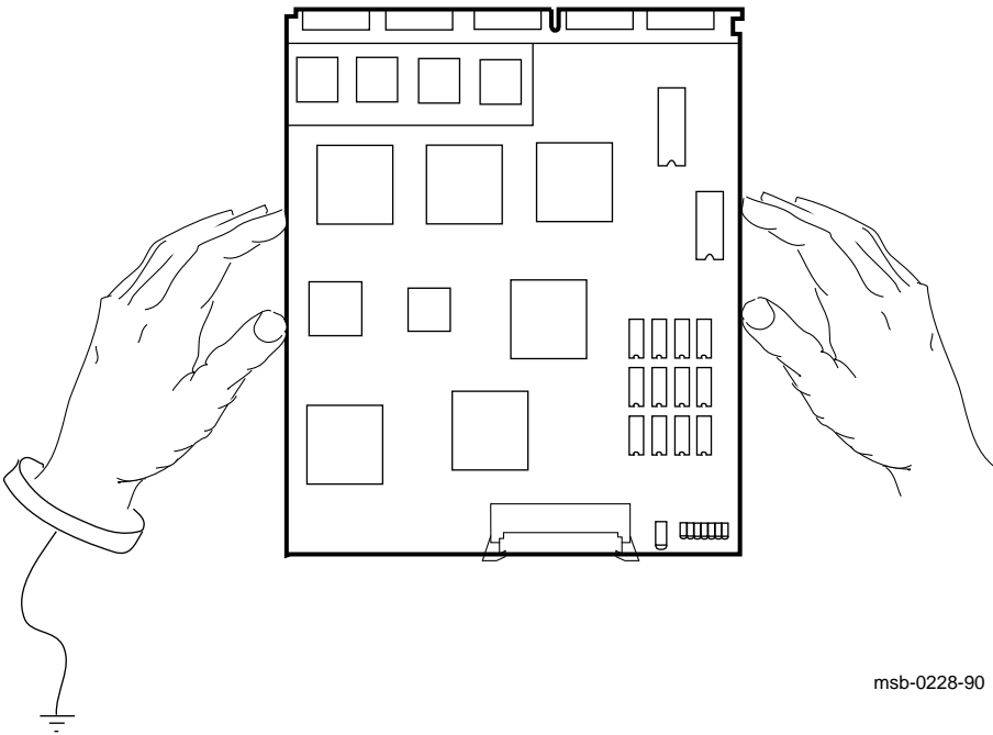
Figure C-1: Holding VAX 6000 Series Processor Modules
