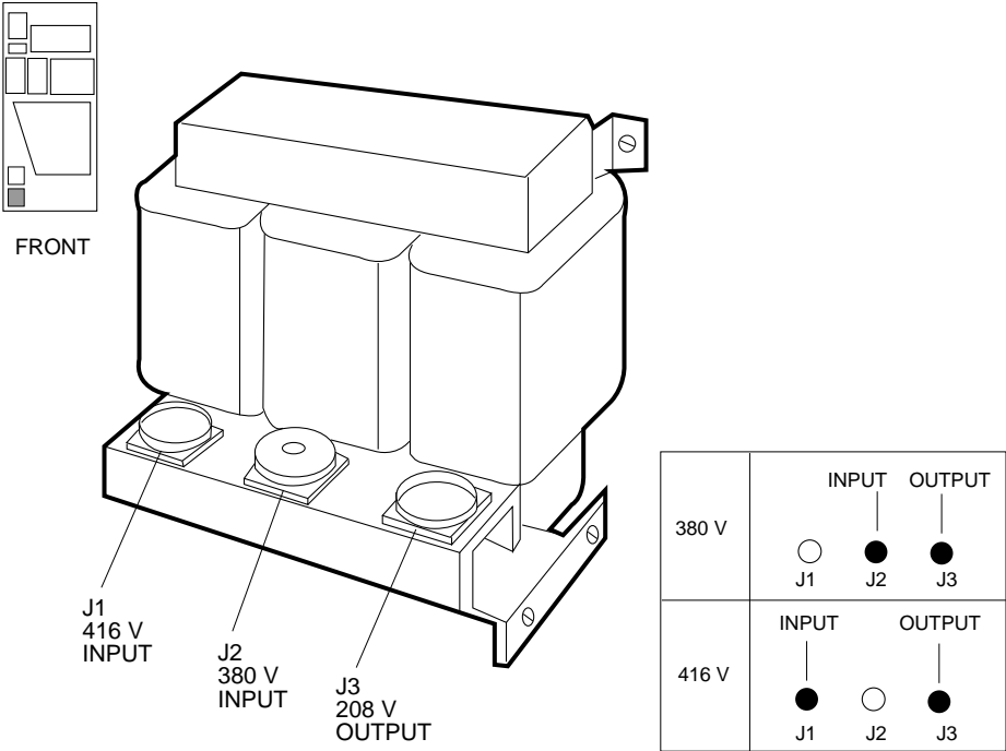
Figure 5-17: 50 Hz Transformer Removal
