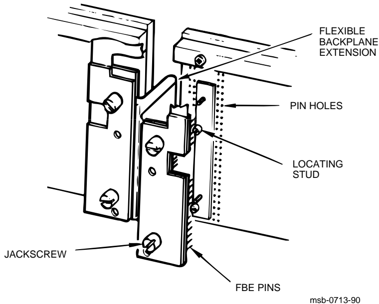
Figure 3-7: VAXBI Flexible Backplane Extension
