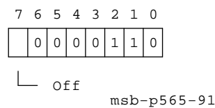
Figure 2–18 Watch Chip CSR B (E018 300B)
