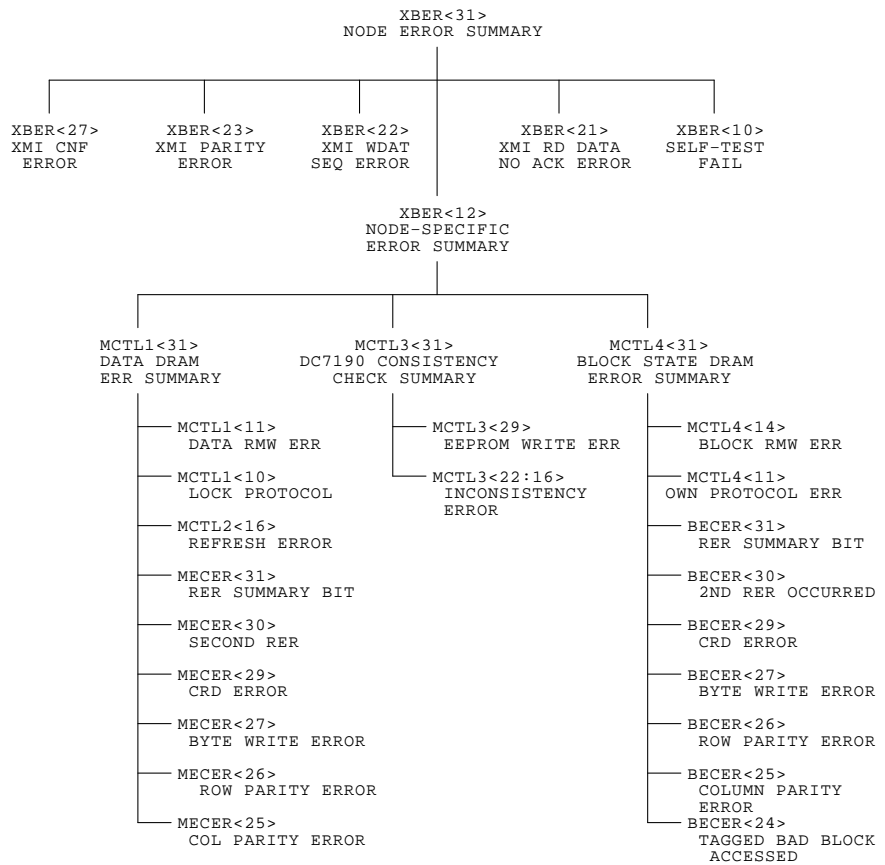
Figure 3–1 Error Bit Hierarchy
