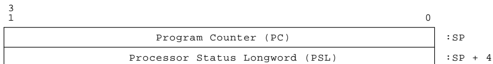
Figure 2-5 Minimum Stack Frame
