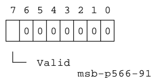
Figure 2–19 Watch Chip CSR D (E018 300D)
