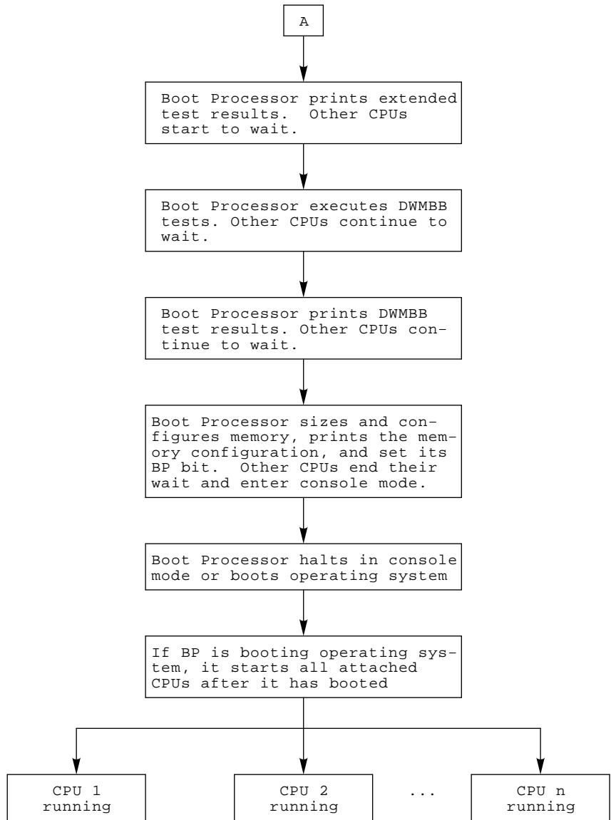
Figure 2-23 (Cont.) Initialization Flowchart
