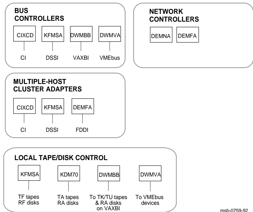
Figure 1-5 Adapters
