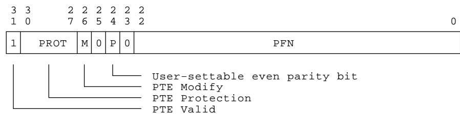
Figure 2–15 PTE Fills from EM Latch
