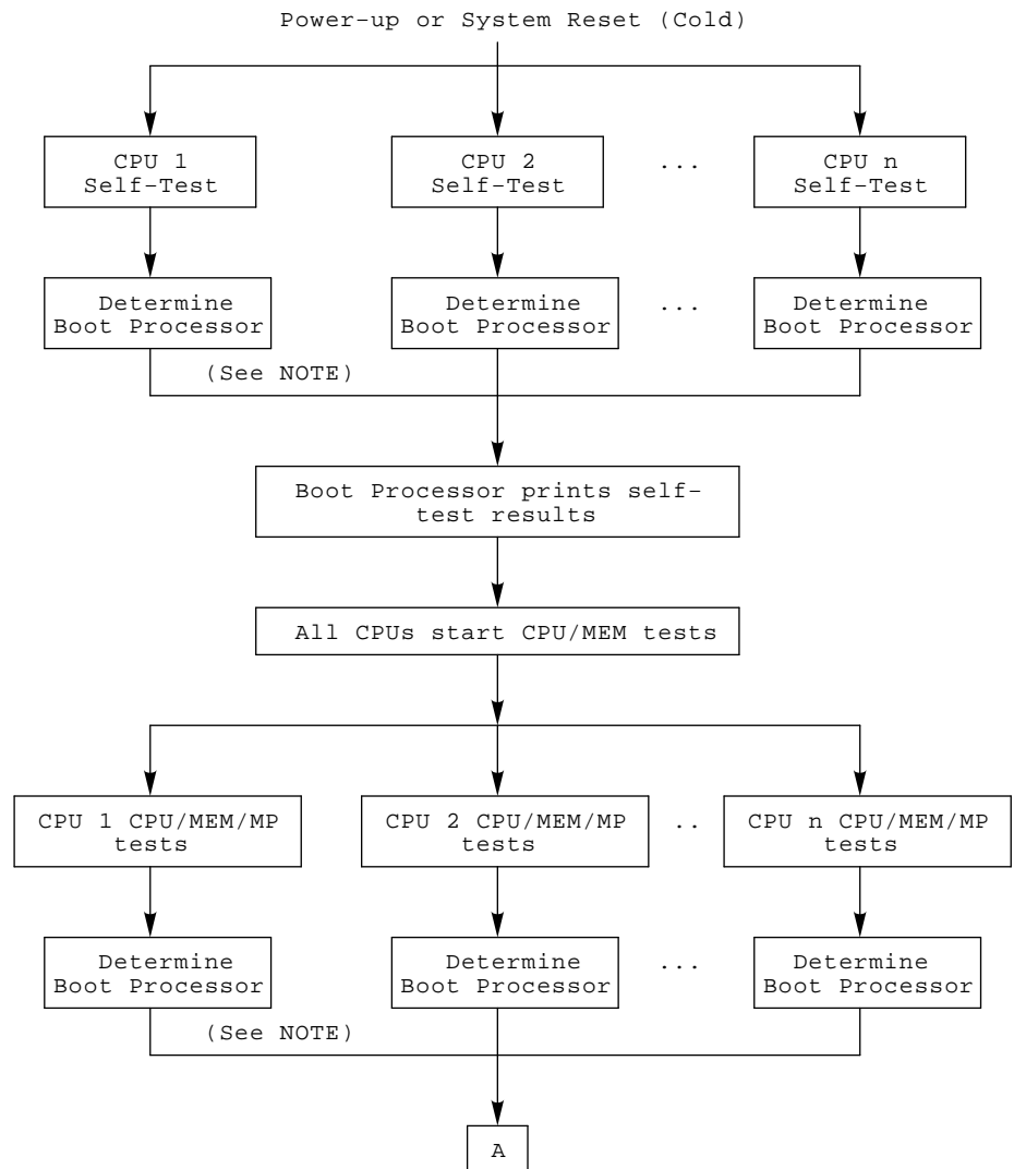
Figure 2-23 Initialization Flowchart
