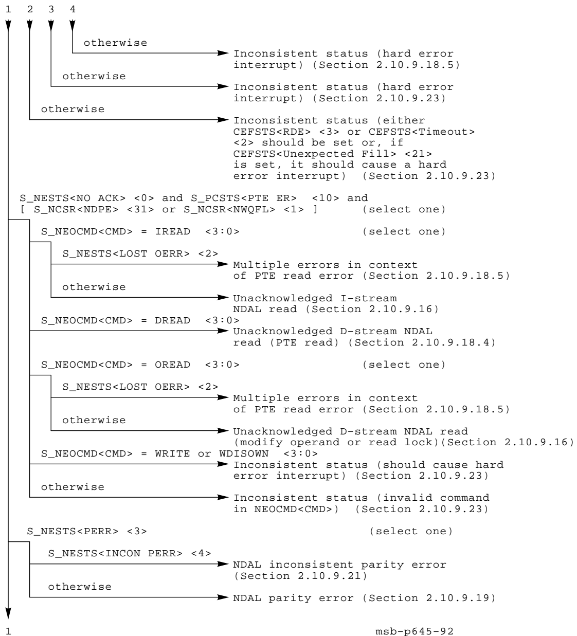
Figure 2–29 (Cont.) Soft Error Interrupt Parse Tree
