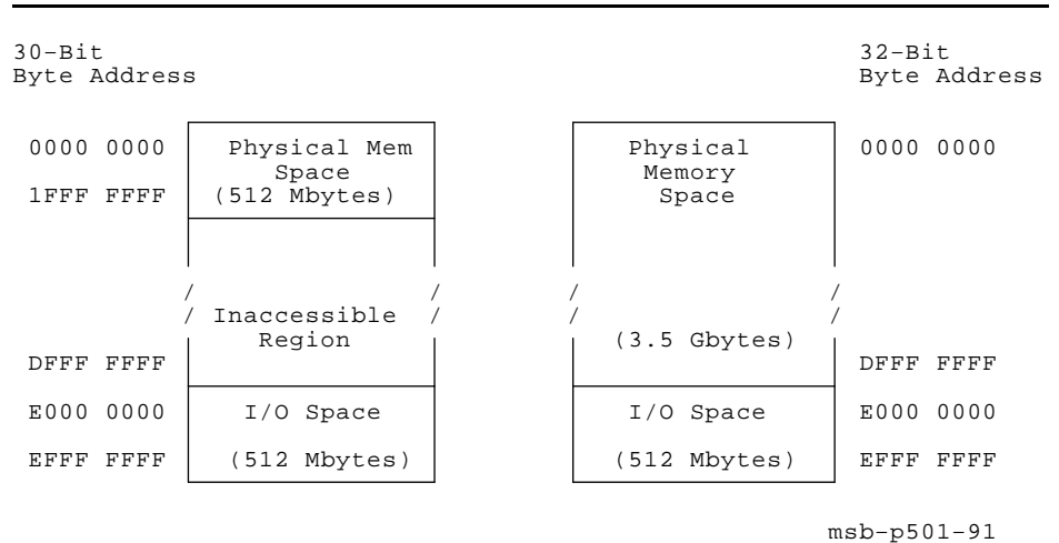
Figure 2-2 Physical Address Space Layout
