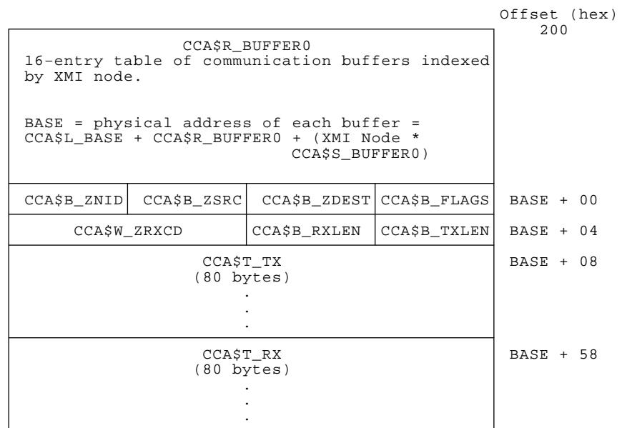
Figure 2–26 Layout of XMI Node Buffers
