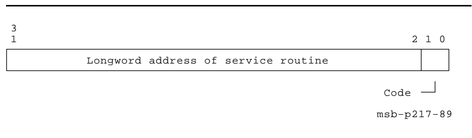
Figure 2–12 System Control Block Vectors
