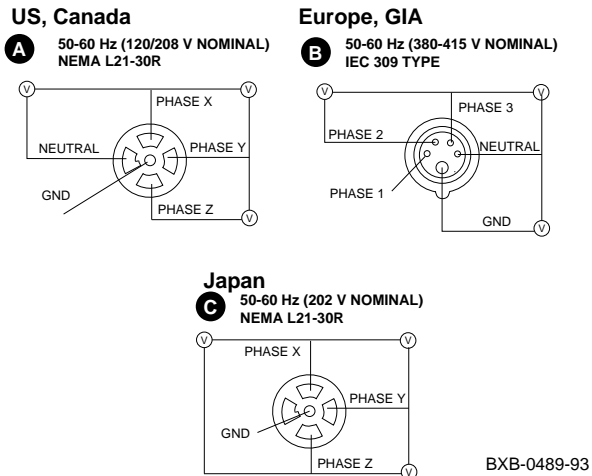
Figure 1-7 Power Receptacles
