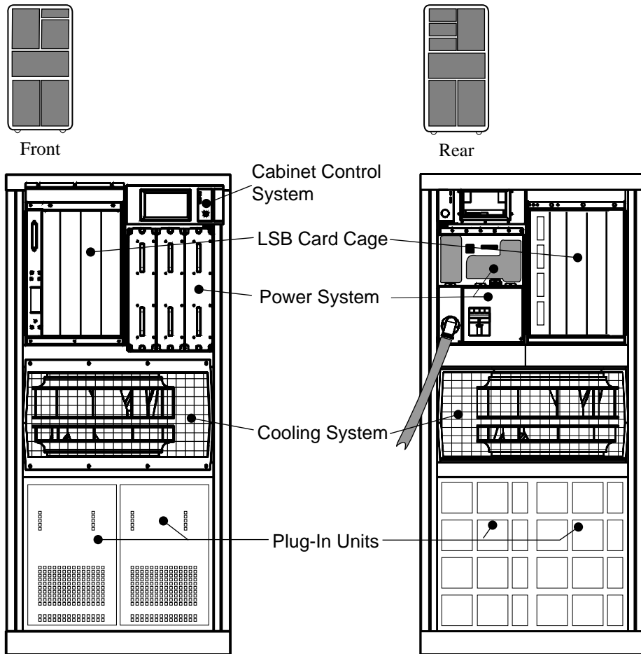
Figure 1-1 The Basic Platform—System Cabinet
