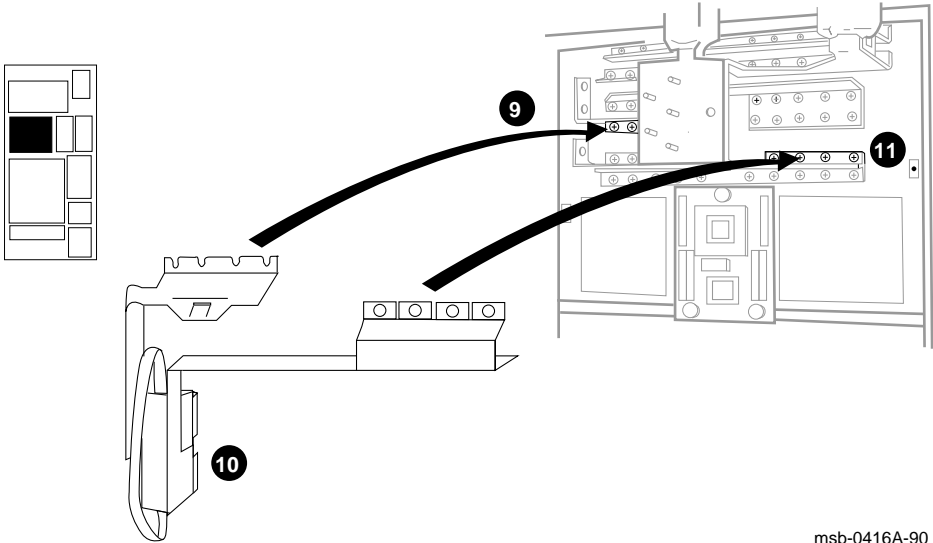
Figure 4-3: Installing the H9657-CX Bus Bar
