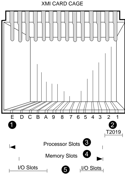
Figure 4-2: XMI Configuration When Using the H9657-CX Kit
