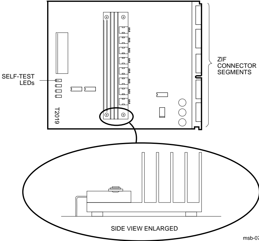
Figure 4-4: Installing the T2019 Power Regulator Module
