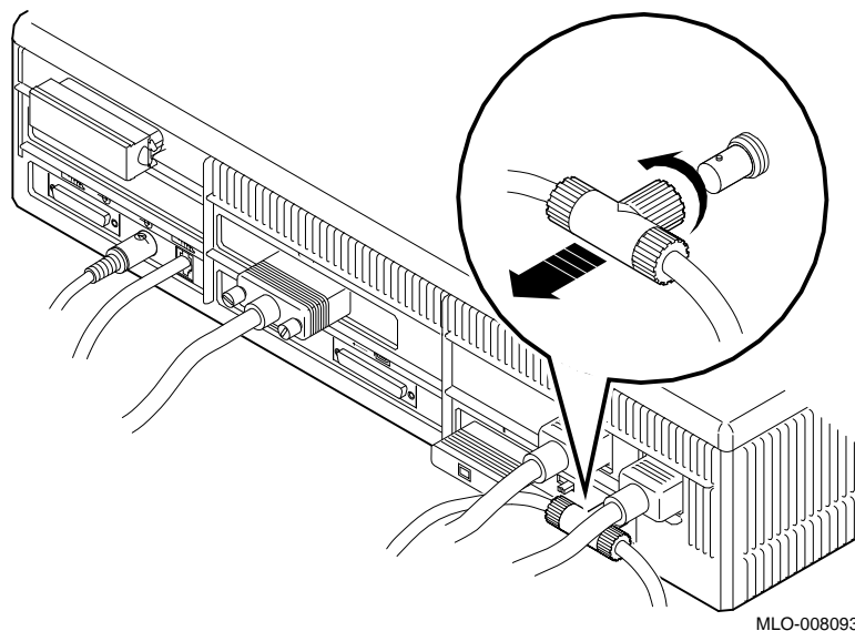
Figure 3-7 Removing the T-connector from the System
