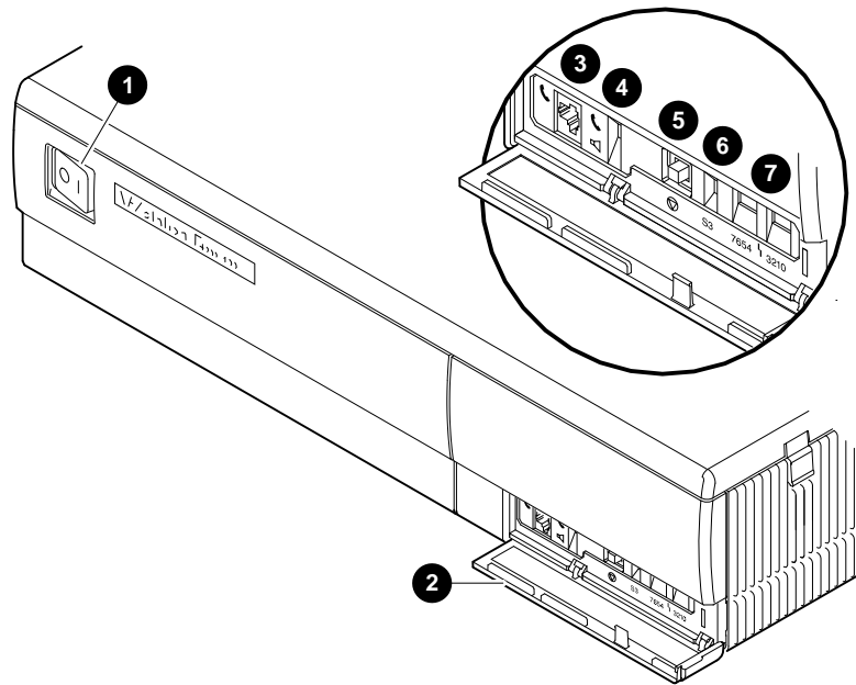
Figure 1-3 Front of System Unit
