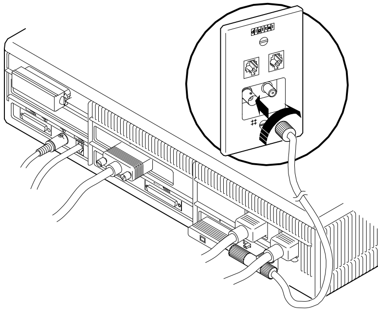
Figure 3-6 Connecting to the DECconnect Faceplate
