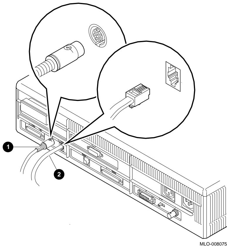
Figure 2-3 Connecting the Mouse and Keyboard
