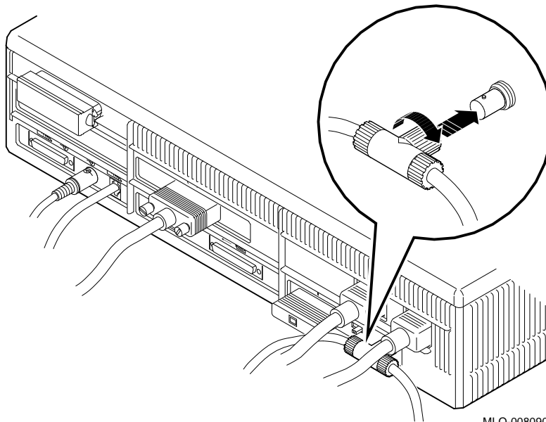
Figure 3-5 Reconnecting ThinWire Cable
