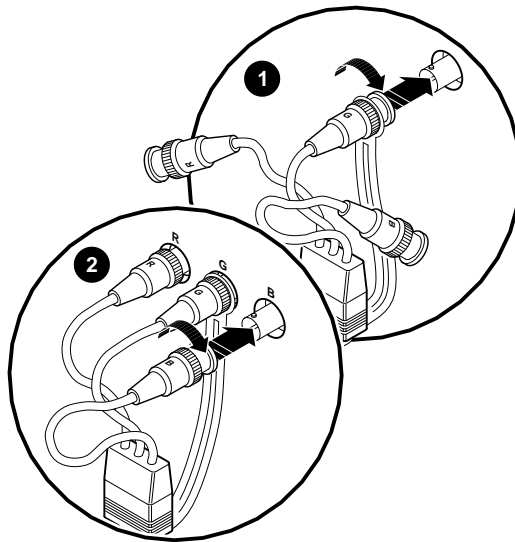
Figure 2-6 Attaching the Monitor Cable to the Monitor
