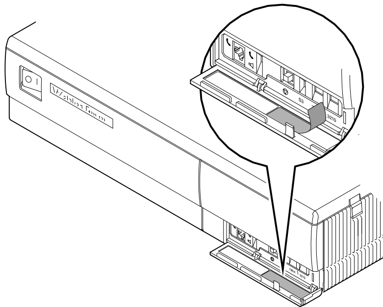
Figure 2-13 Attaching the Network Label
