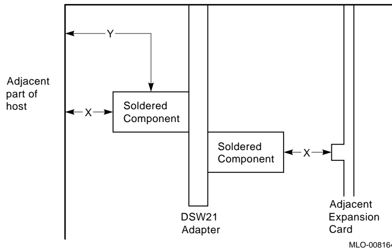
Figure B-1 Creepage Distance
