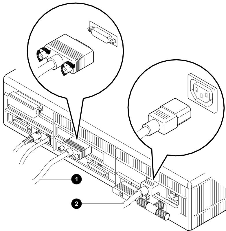
Figure 2-4 Attaching the Monitor Cable
