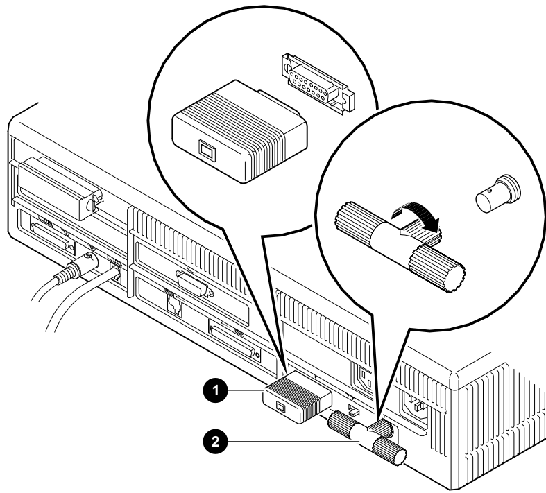
Figure 2-2 Attaching the Loopback and T-connector
