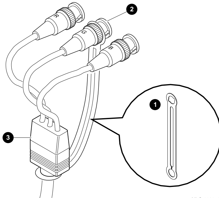
Figure 2-5 Attaching the Universal Strain Relief Strap
