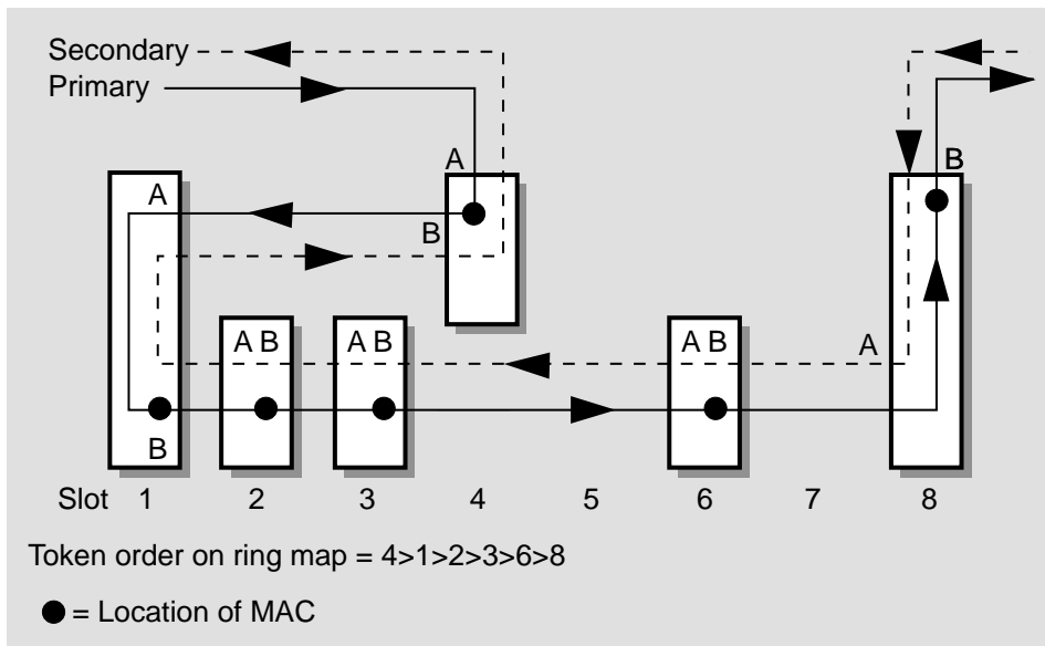
Figure 3-30: Token Flow through Dual Ringed DEChub 900 Modules
