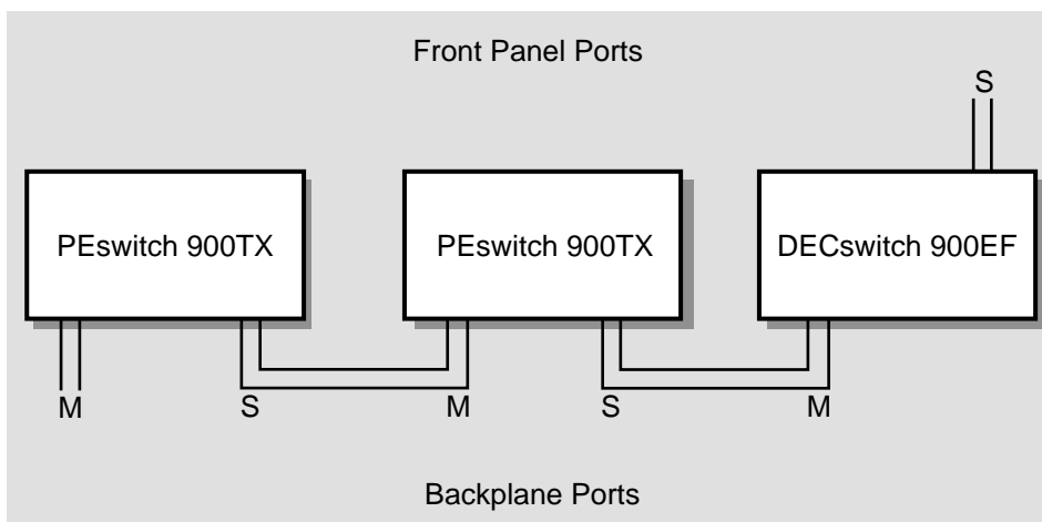
Figure 3-14: Tree Connections to an External FDDI Network
