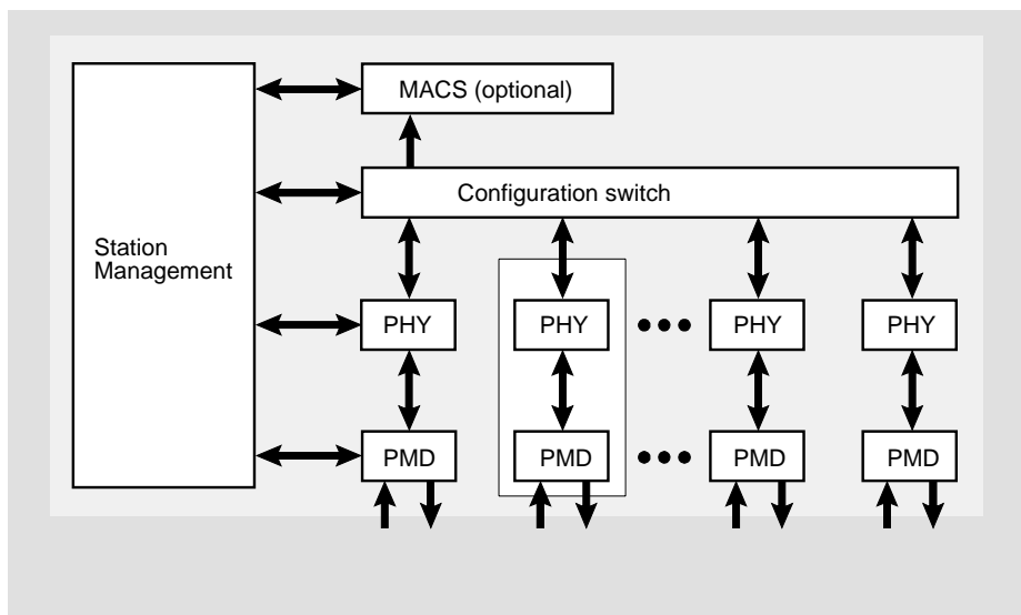
Figure 1-4: Concentrator Architecture
