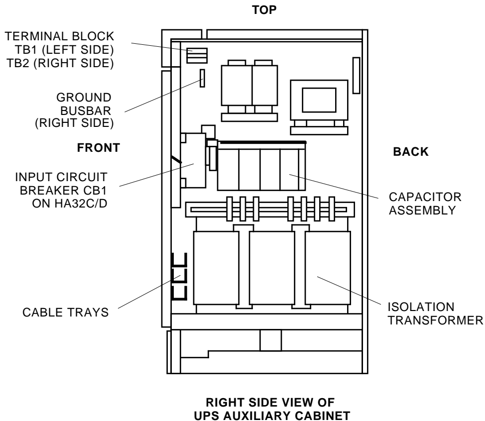
Figure 4-7 UPS Auxiliary Cabinet Cable Trays
