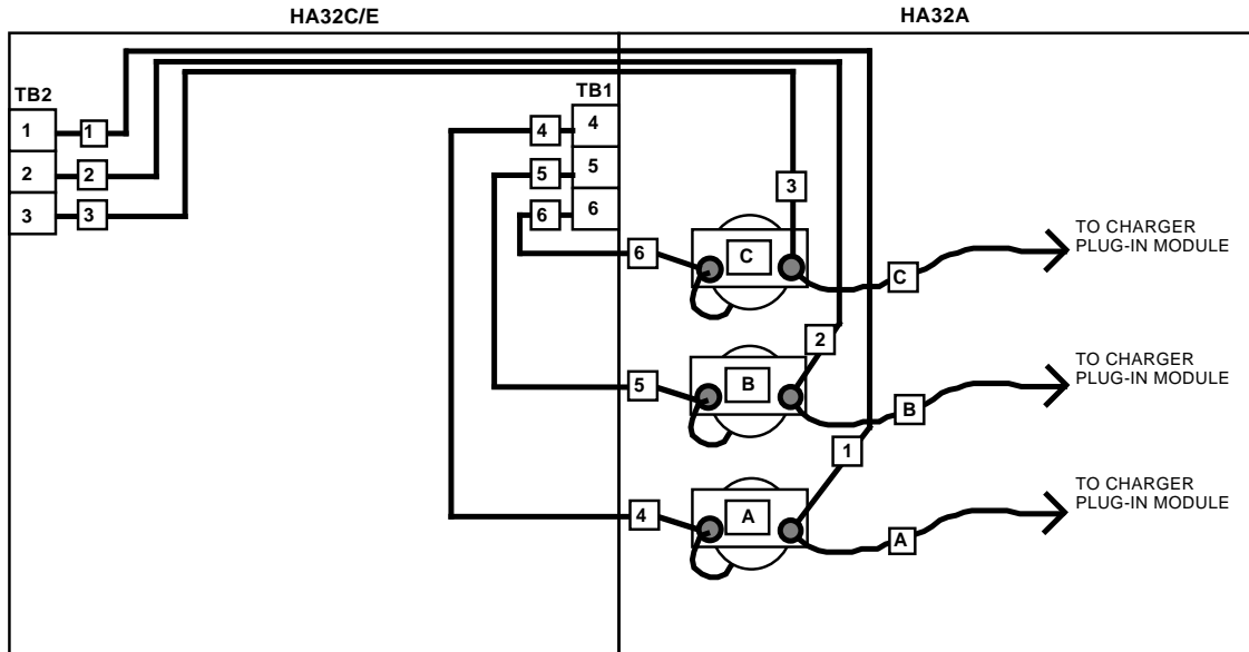
Figure 4-14 UPS Cabinet with Input Harmonic Current Filter Installed
