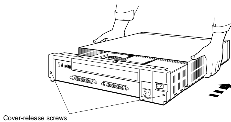
Figure 2 Removing the Expansion Box Cover
