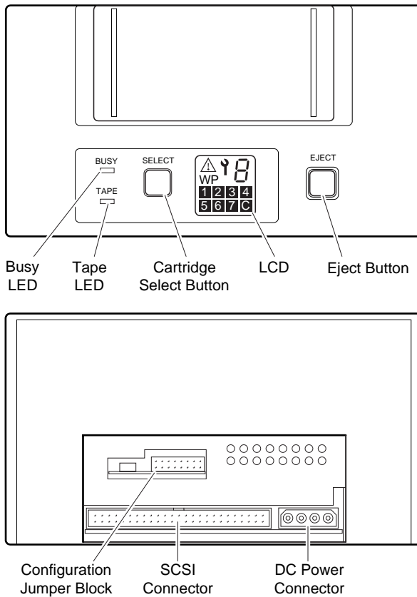
Figure 7-1 Model TLZ9L-AA (Front and Rear View)
