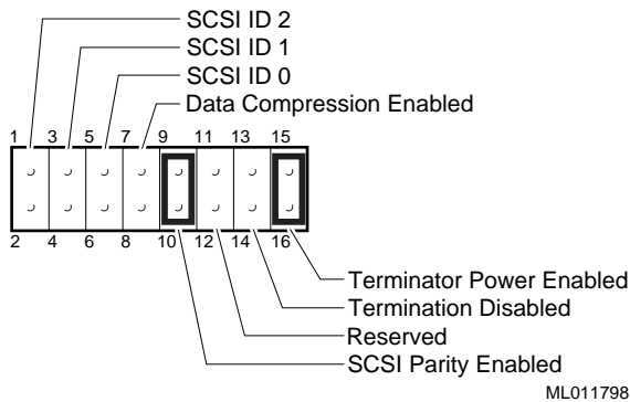
Figure 3-1 Configuration Jumper Block
