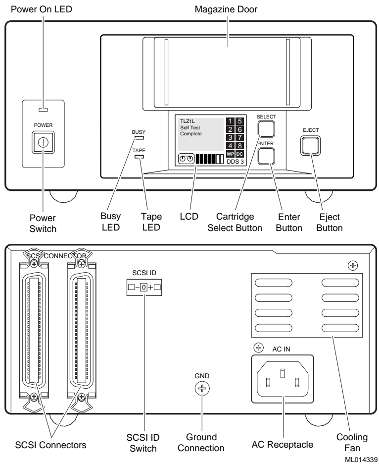
Figure 7-5 Model DS-TLZ1L-DB (Front and Rear View)
