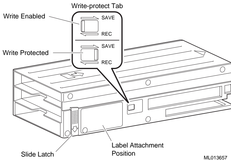
Figure 7-7 TLZ9L/TLZ1L Cassette Magazine
