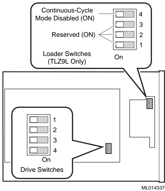
Figure 7-2 Model TLZ9L-AA/TLZ1L-AA Bottom View
