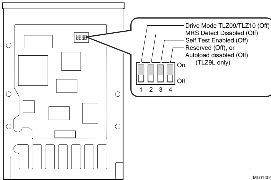
Figure 1-4 TLZ09/TLZ10 Chassis - Underside with Switch Pack
