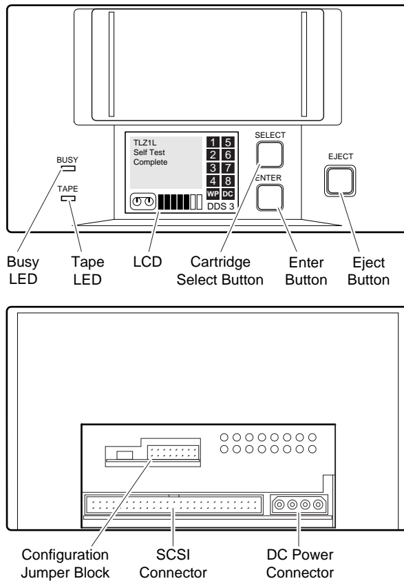
Figure 7-3 Model TLZ1L-AA (Front and Rear View)
