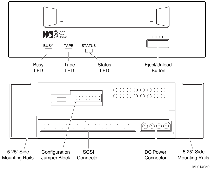
Figure 1-3 Model TLZ09-BA/BB and TLZ10-BB (5.25-inch Chassis)
