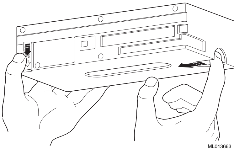
Figure 7-14 Unloading Cartridges From the Magazine
