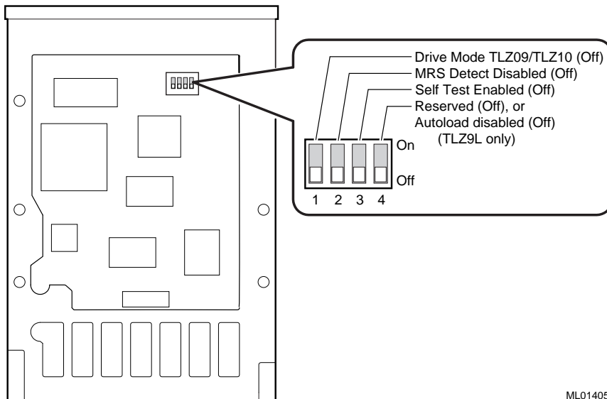
Figure 3-2 Drive Switch Settings
