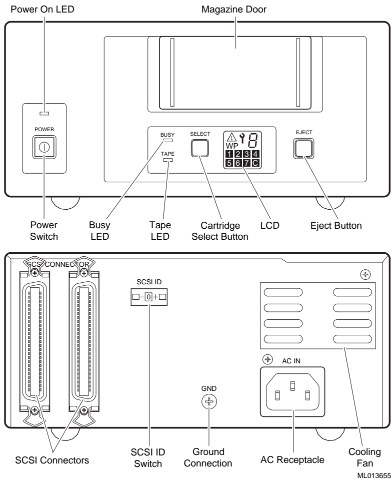
Figure 7-4 Model TLZ9L-DB (Front and Rear View)
