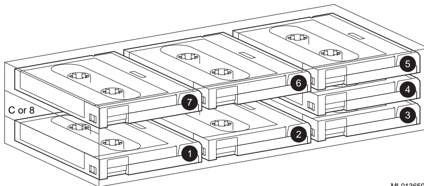
Figure 7-10 Seven Cartridge Mode
