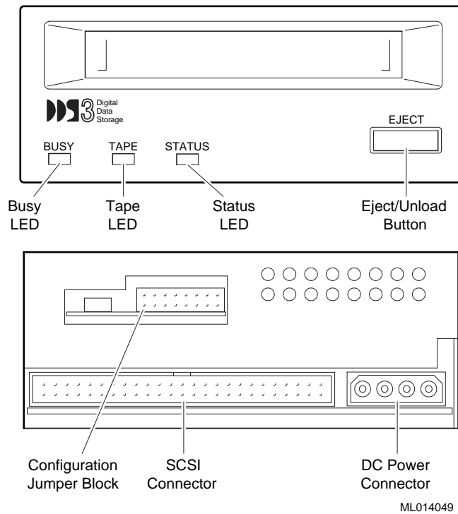
Figure 1-2 Model TLZ09-AA/AB and TLZ10-AB (3.5-inch Chassis)
