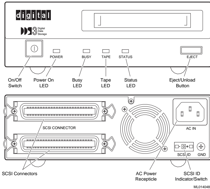
Figure 1-1 Model TLZ09-DA/DB and DS-TLZ10-DB (Tabletop)
