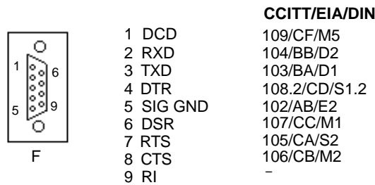
Figure A-2 9-Pin EIA 232 Port
