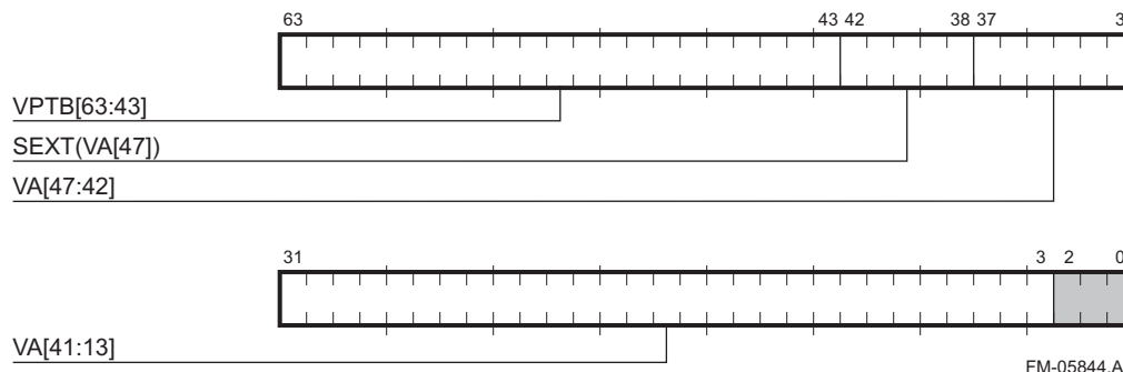
Figure 5–13 Instruction Virtual Address Format Register (VA_48 = 1, VA_FORM_32 = 0)
