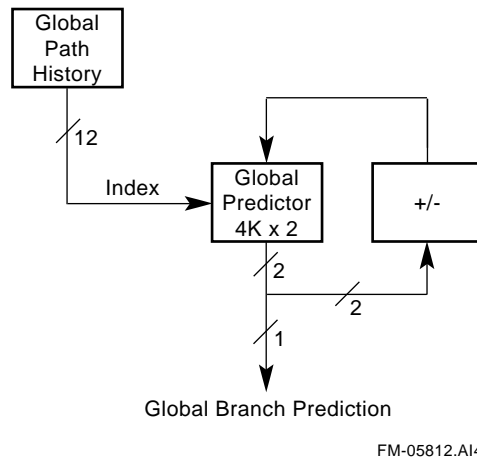
Figure 2–4 Global Predictor
