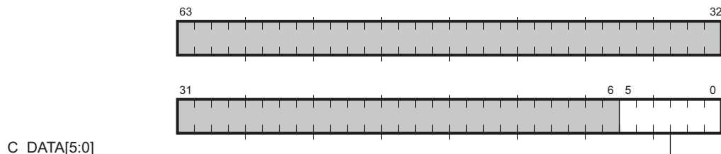
Figure 5–34 Cbox Data Register
