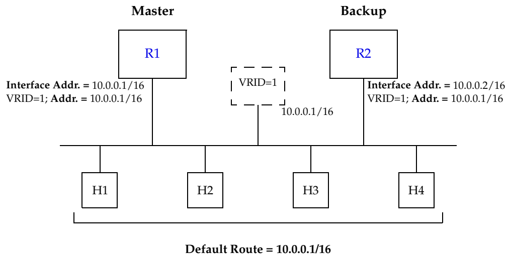
Figure 17. Basic VRRP Configuration
