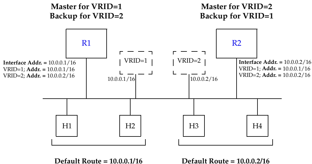
Figure 18. Symmetrical VRRP Configuration
