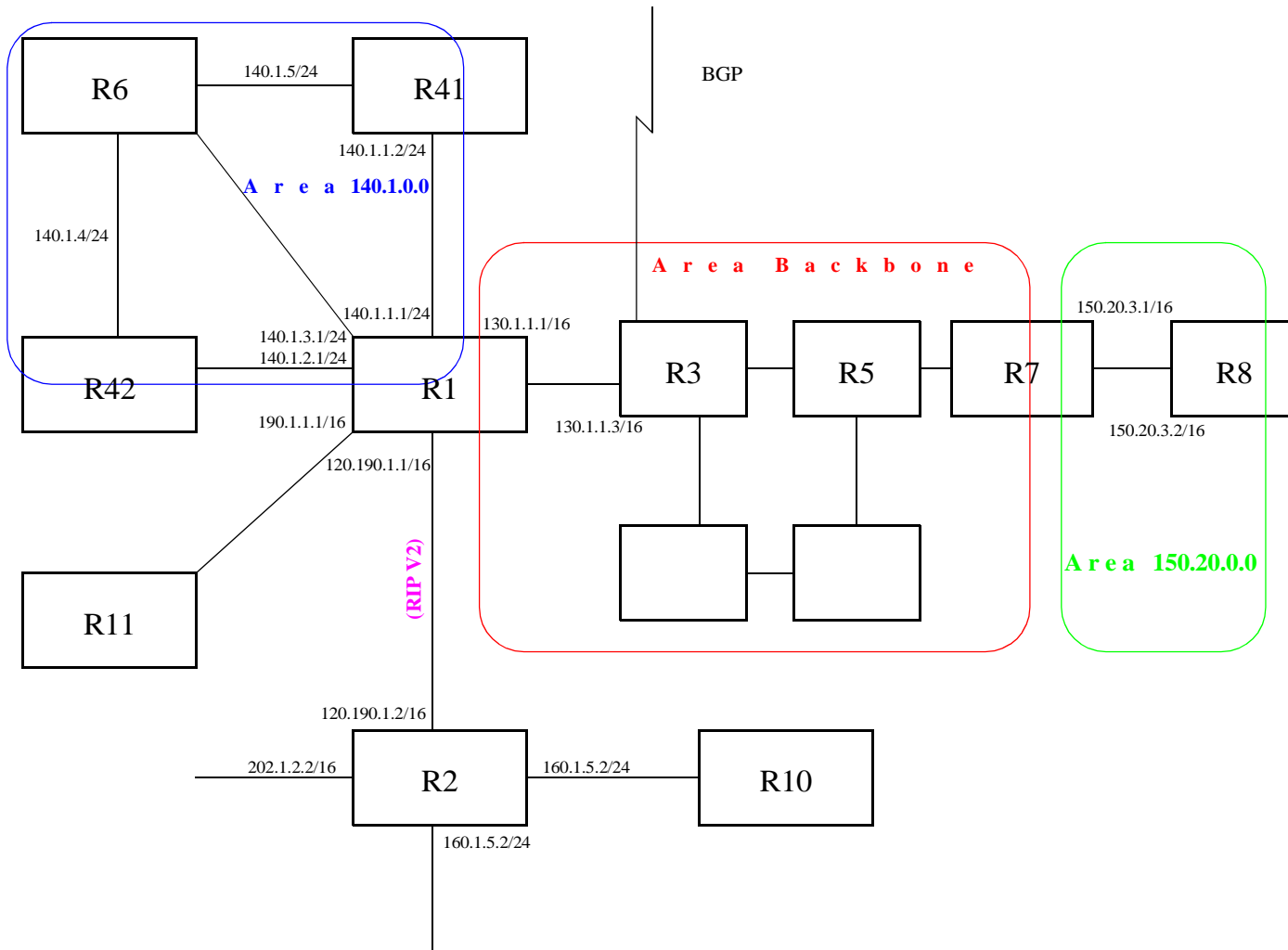
Figure 1. Exporting to OSPF
