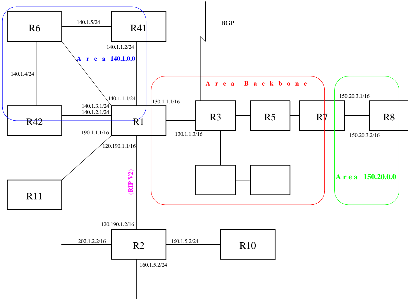
Figure 12: Exporting to OSPF
