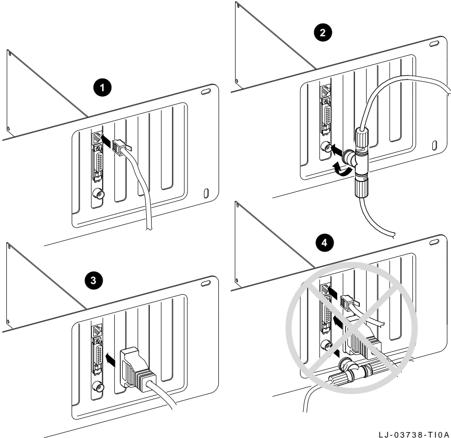
Figure 3-5 Connecting to the Ethernet Network
