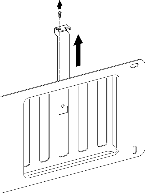
Figure 3-3 Removing the Slot Cover
