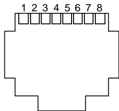
Figure B-1 RJ-45 Connector (Front View)
