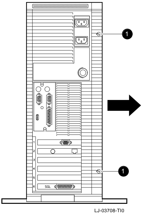
Figure 3-1 Removing the System Unit Outside Cover
