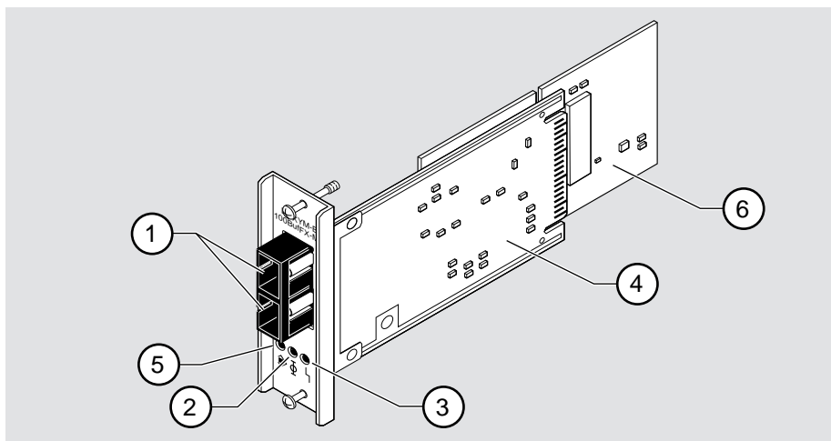
Figure 1-3: 100BufFX Components
