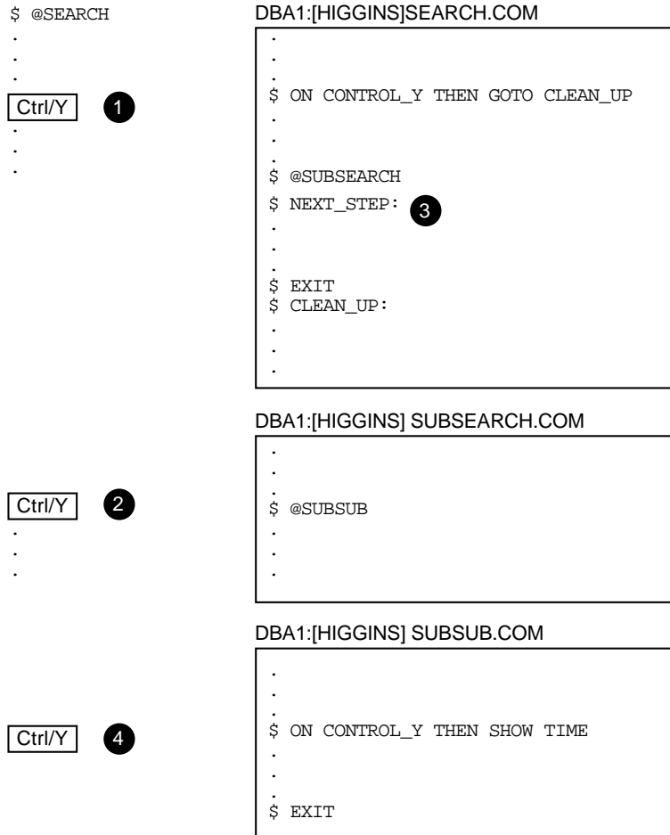
Figure 15–3 Ctrl/Y in Nested Procedures
