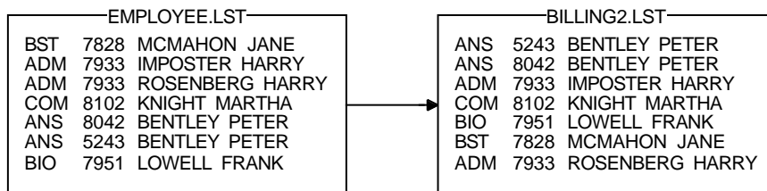
Figure 11–5 Sorting with Multiple Key Fields
