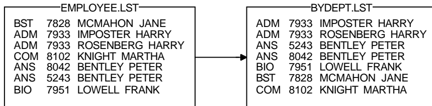
Figure 11–4 Sorting with Default Key Records
