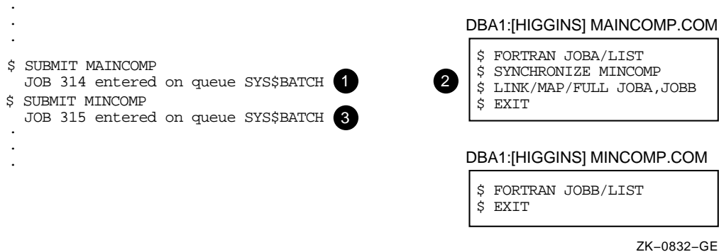
Figure 18–1 Synchronizing Batch Job Execution
