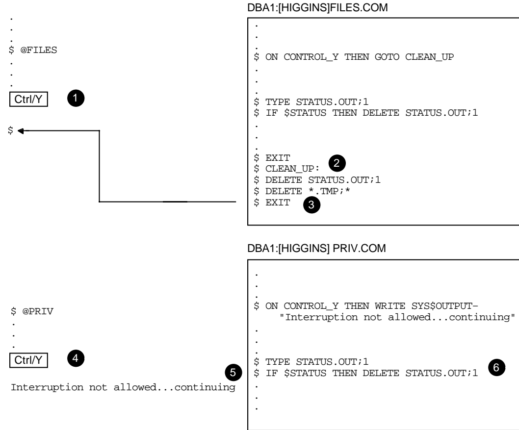
Figure 15–2 Flow of Execution Following Ctrl/Y Action
