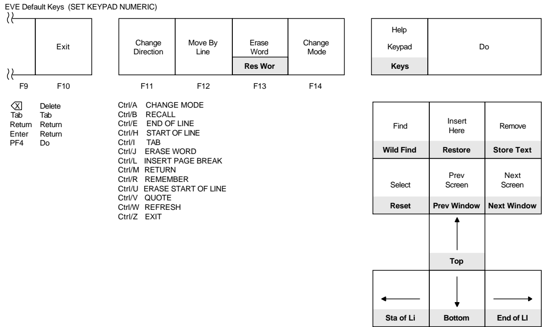
Figure 8–1 EVE Keys — VT200, VT300, and VT400 Series Terminals
