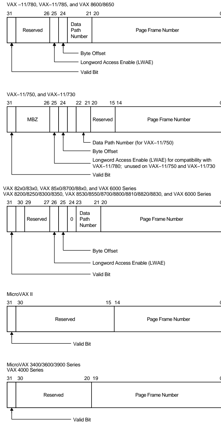
Figure 14-1 UNIBUS and Q22-bus Map Registers
