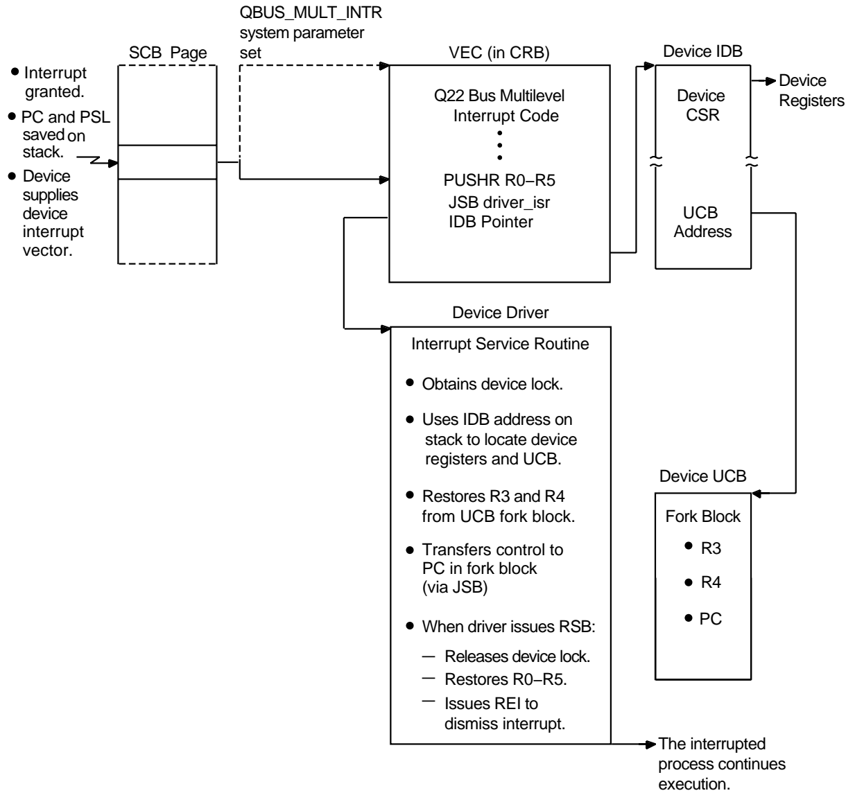
Figure 14-5 Direct-Vector Interrupt Dispatching
