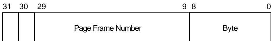
Figure 21–1 Format of a Physical Address
