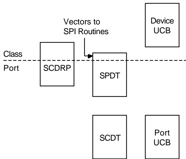
Figure 17–4 SCSI Class/Port Data Structures
