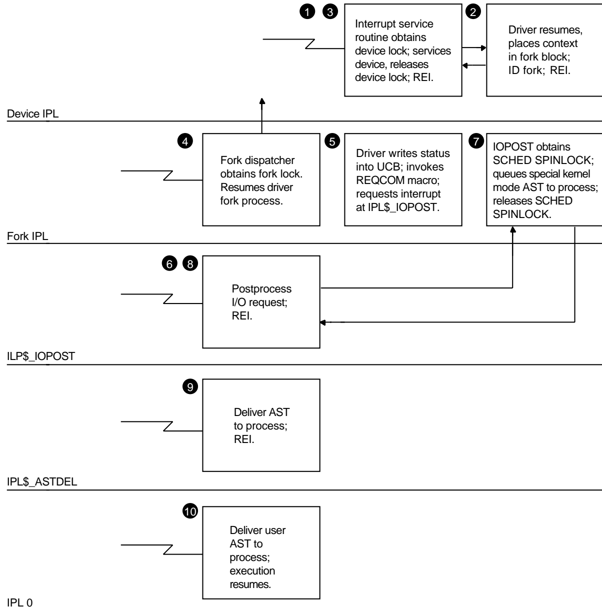
Figure 3–2 Synchronizing I/O Request Completion
