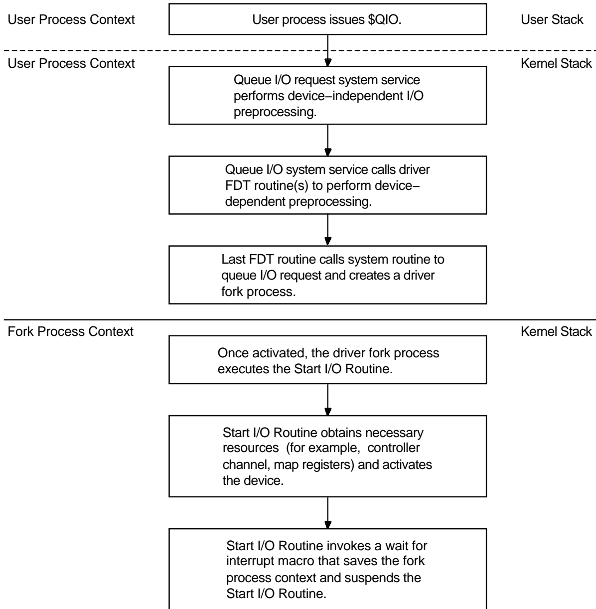
Figure 4-1 Sequence of Driver Execution
