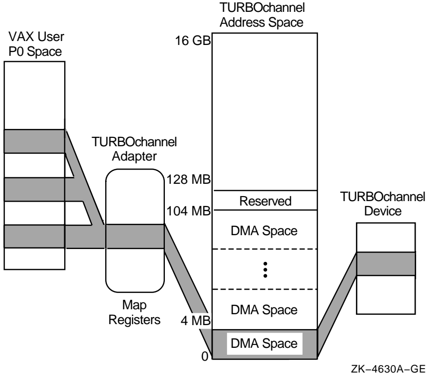
Figure 19-3 TURBOchannel DMA to a VAX Host
