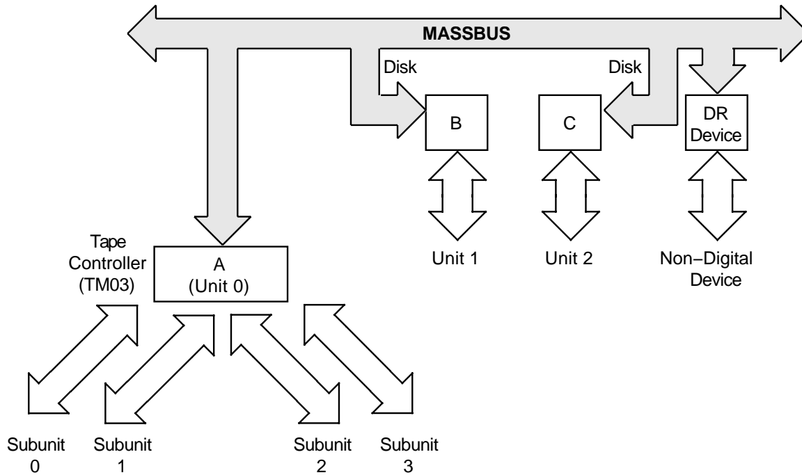
Figure 15–1 MASSBUS Configuration
