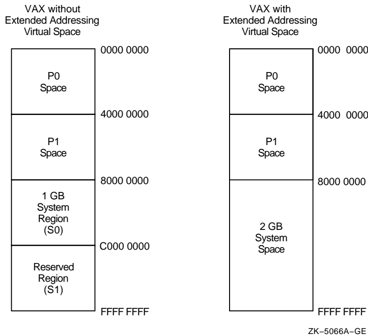
Figure 1–3 Virtual Address Space for VAXes
