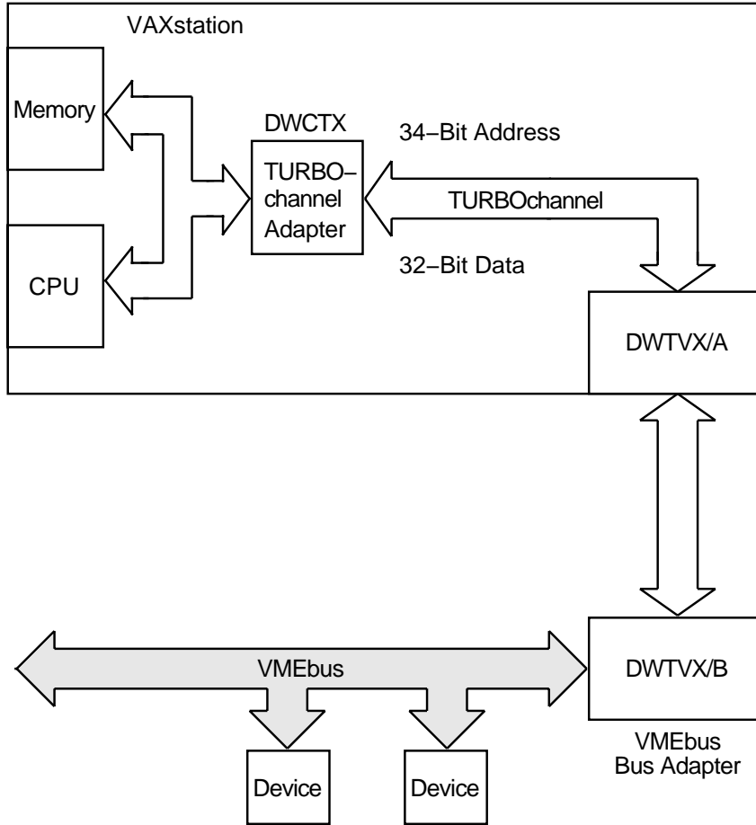
Figure 20-1 TURBOchannel-Based VAXstation with a VMEbus Subsystem
