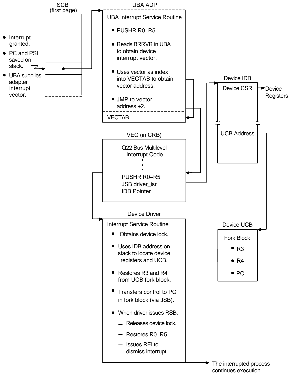
Figure 14-6 Non-Direct-Vector Interrupt Dispatching
