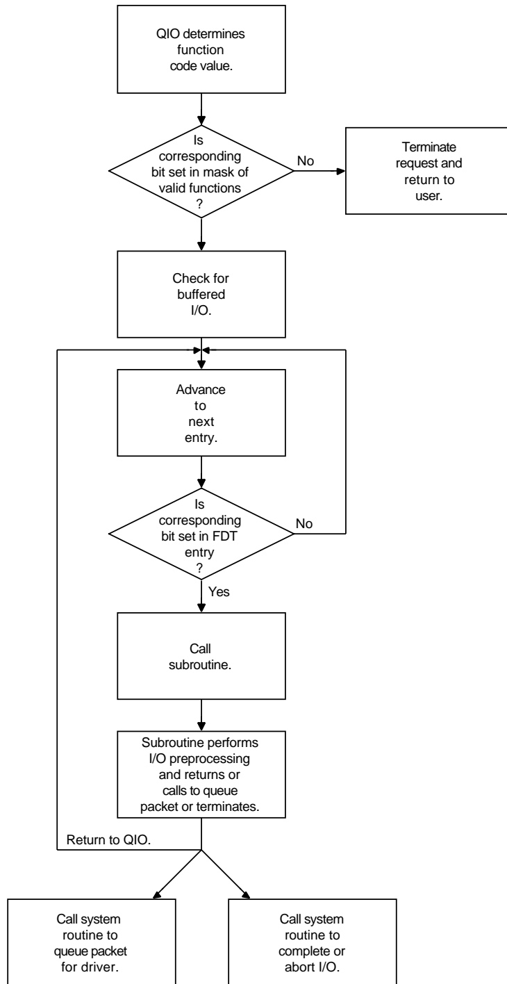
Figure 4–6 FDT Routines and I/O Preprocessing
