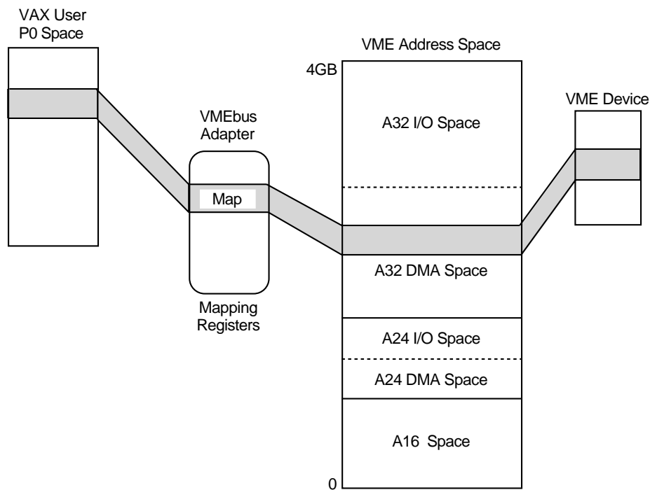
Figure 20-4 VMEbus DMA to and from VAX Host
