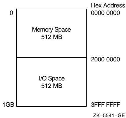
Figure 16–1 VAXBI Address Space
