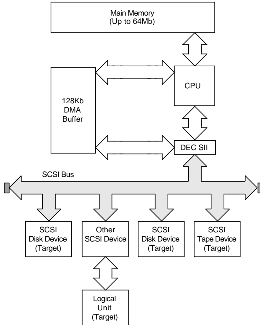
Figure 1-10 VAXstation 3520/3540 System Architecture
