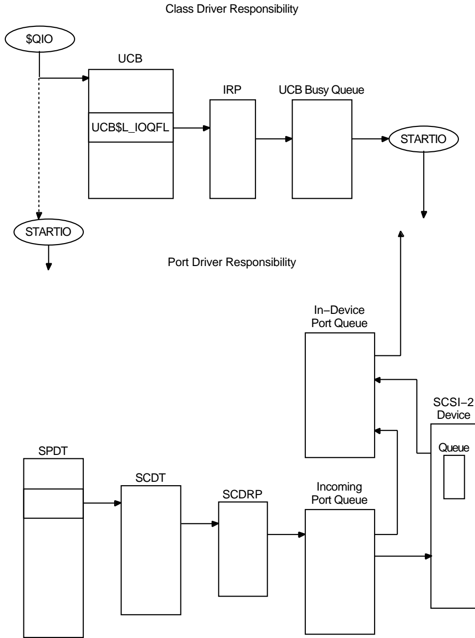
Figure 17–5 Class/Port Tagged Command Queuing Model
