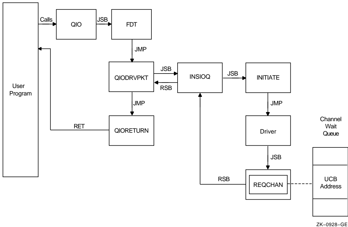
Figure 8-1 Inserting a UCB into the Channel Wait Queue
