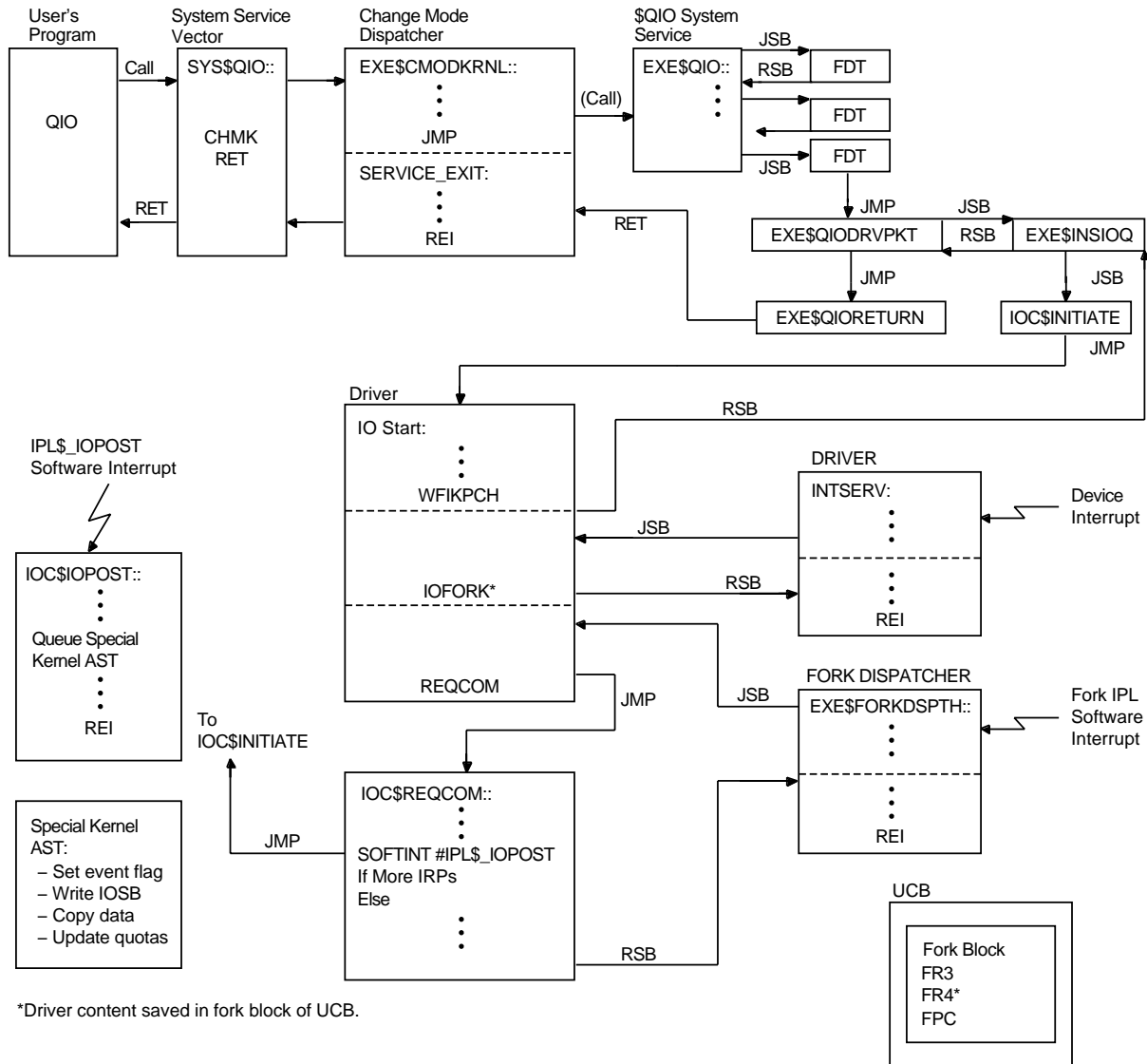
Figure 4–2 Detailed Sequence of System I/O Processing
