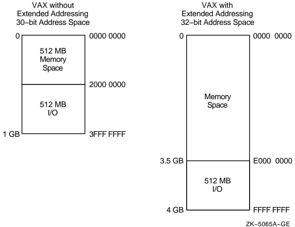
Figure 1–2 Physical Address Space for VAXBI Based Processors
