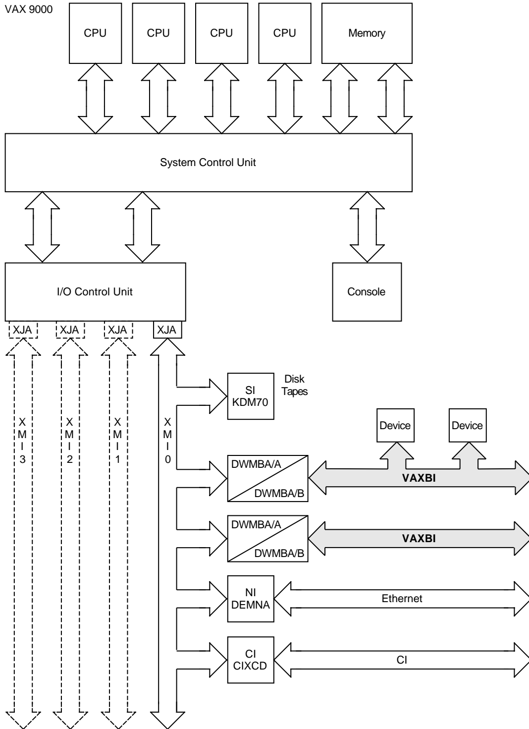
Figure 1-6 SCU/XMI-Based Systems Architecture
