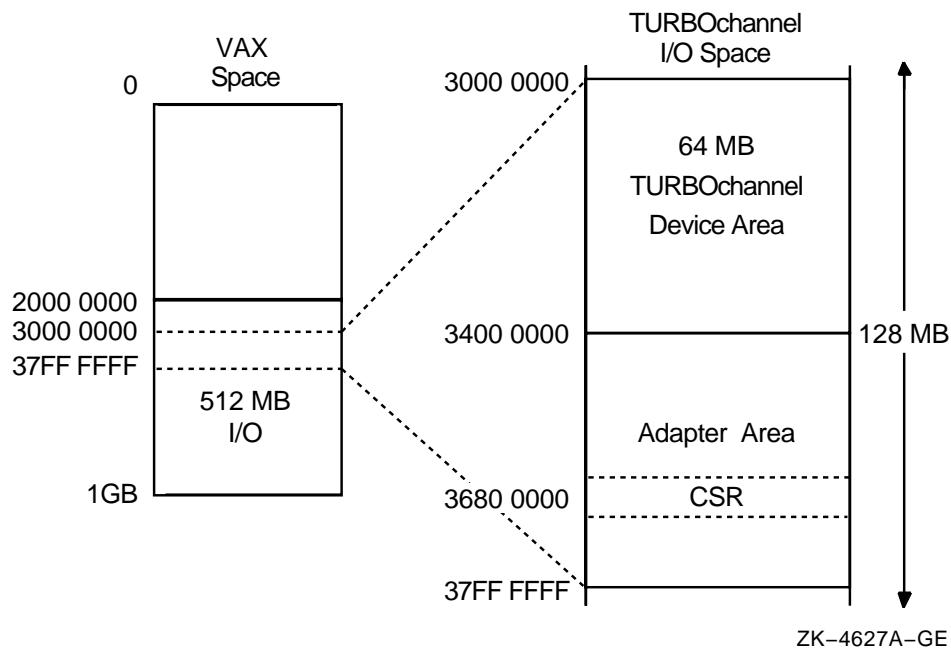
Figure 19–2 TURBOchannel Adapter Space for the VAXstation CPU
