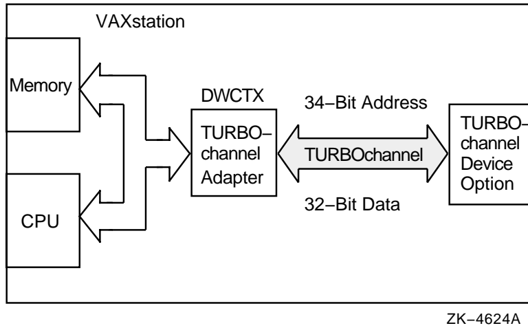
Figure 19–2 TURBOchannel Adapter Space for the VAXstation CPU
