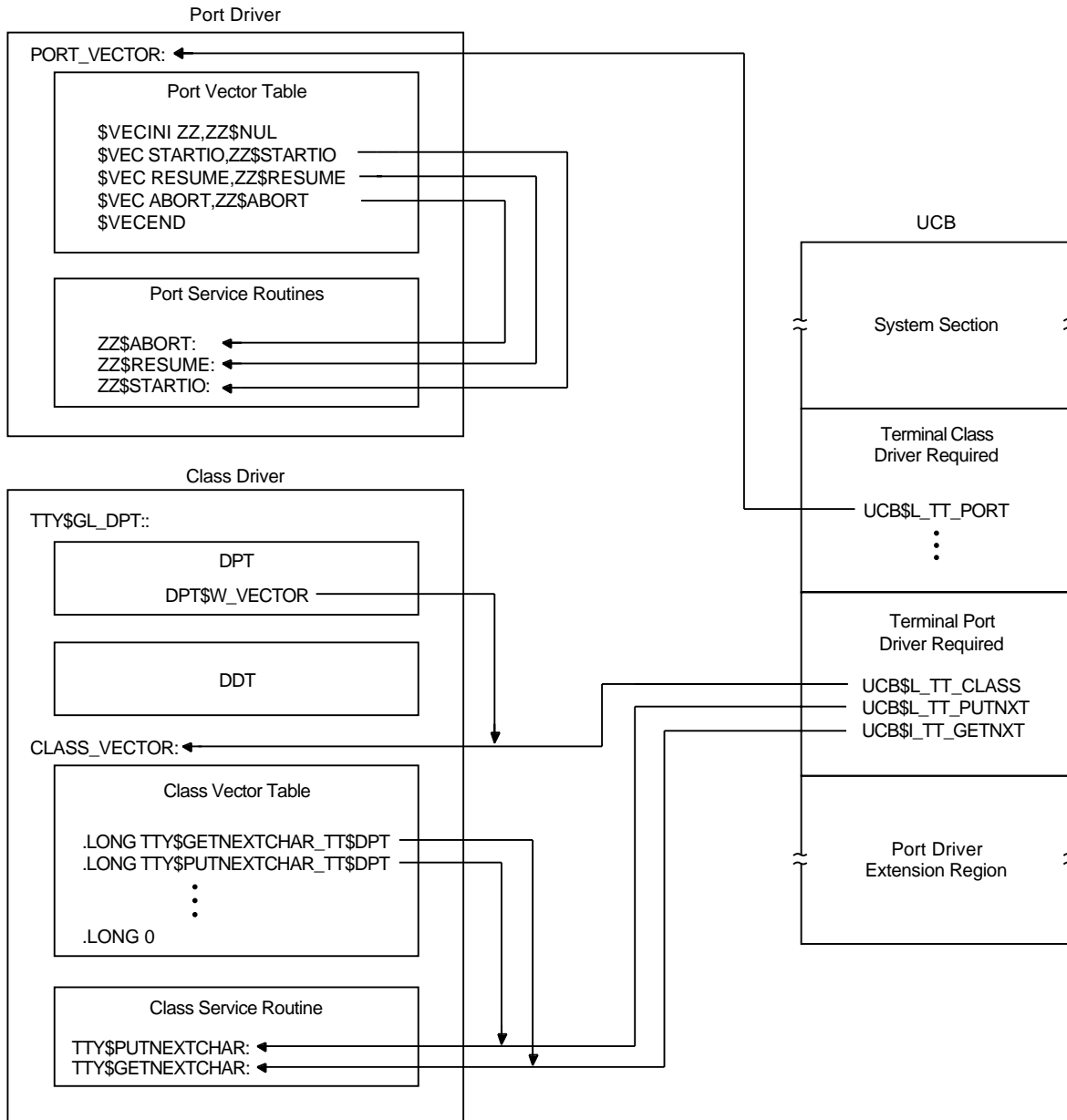
Figure 18–6 Terminal Class/Port Driver Binding
