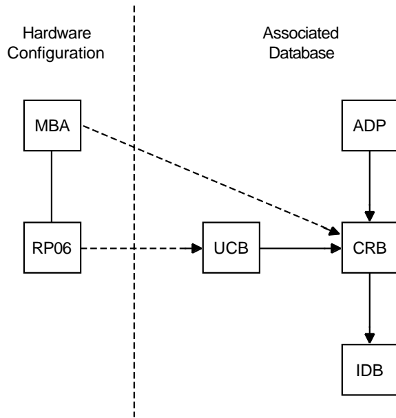
Figure 15-4 I/O Database for MASSBUS Disk Unit
