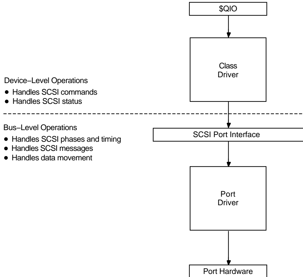
Figure 17-1 SCSI Class/Port Interface
