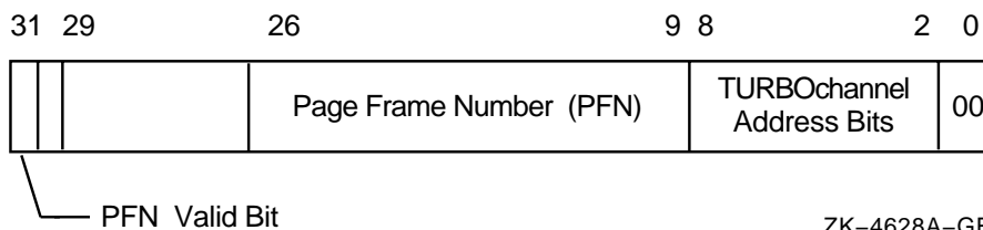
Figure 19-4 TURBOchannel Map Register
