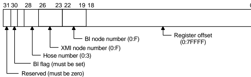
Figure 16-5 VAXBI Pseudo CSR Address (PCA)
