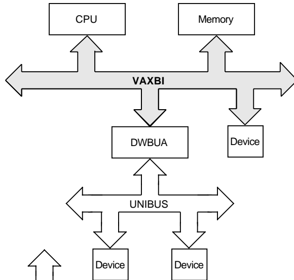
Figure 1-5 VAXBI Based Systems
