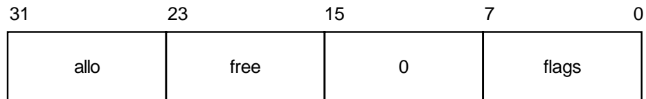
Figure 13–1 Format of the POOLCHECK System Parameter
