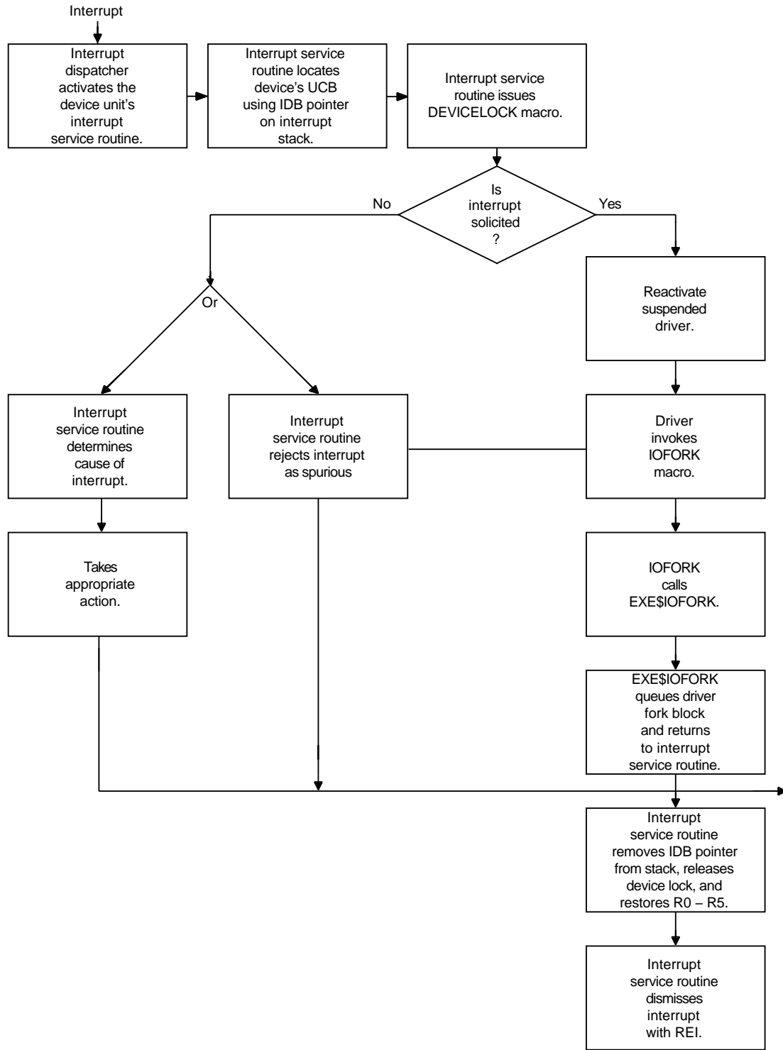
Figure 9-1 Flow of Interrupt Servicing
