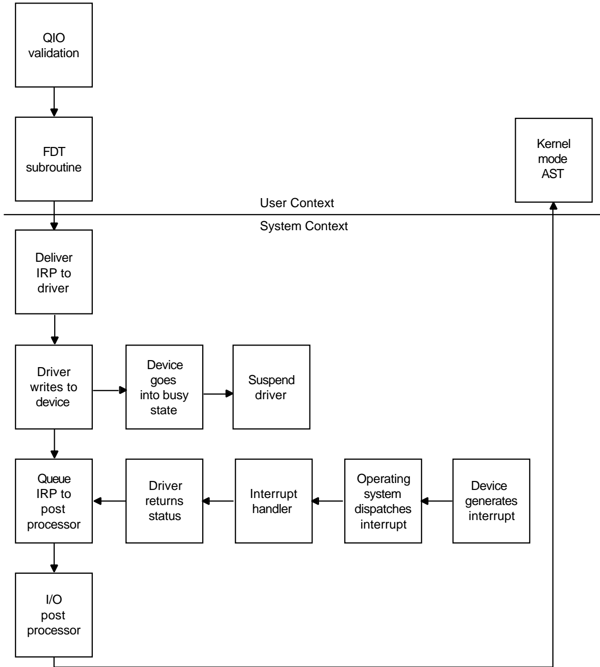
Figure 2-1 A Printer Write Function
