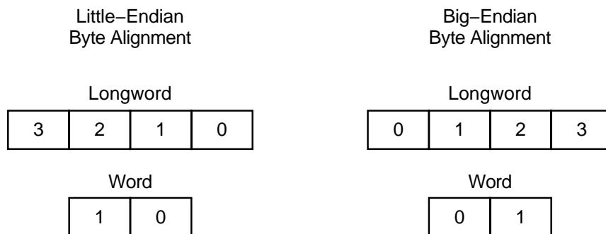
Figure 20–3 Little-Endian Versus Big-Endian Byte Alignment
