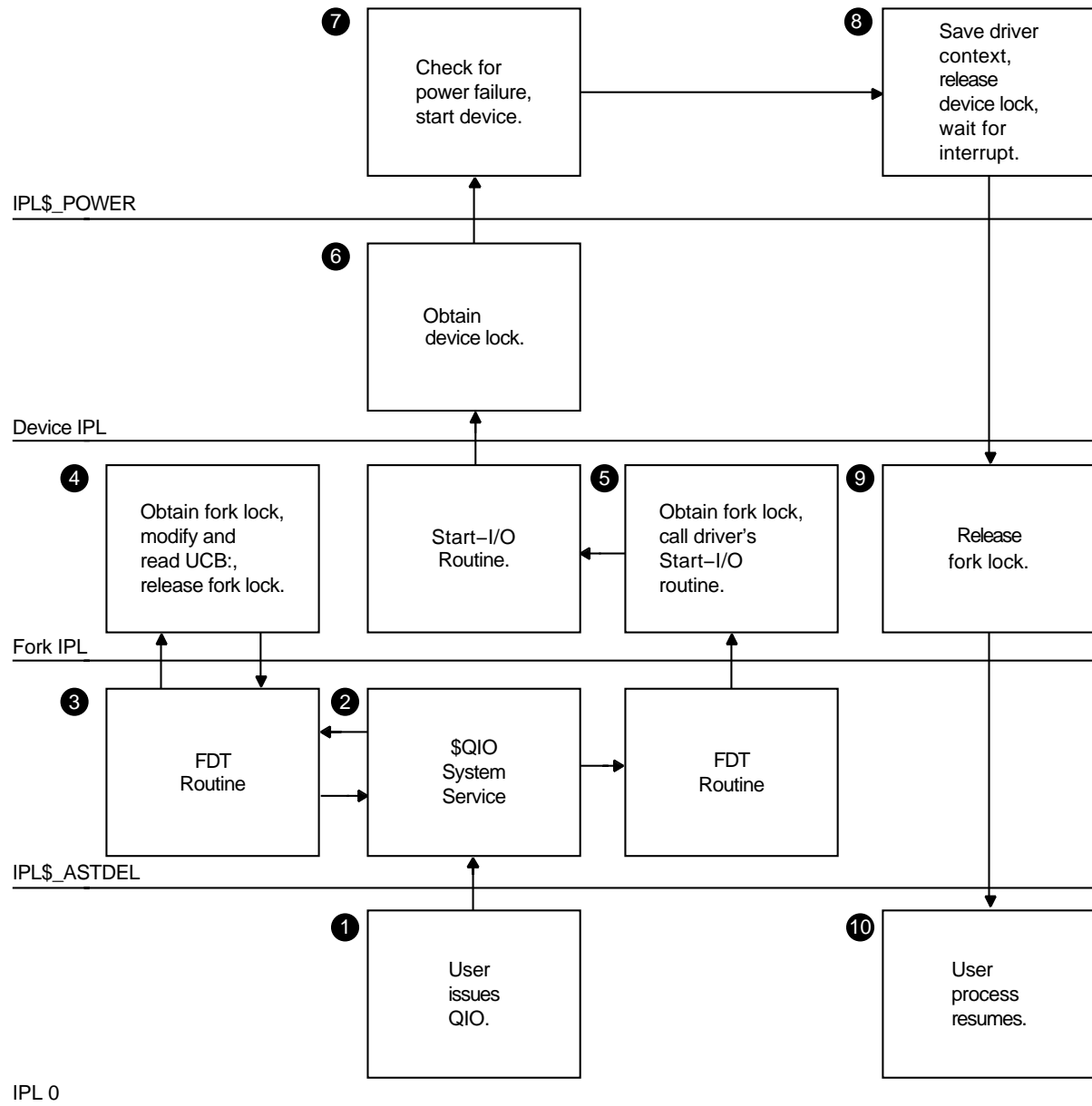
Figure 3–1 Synchronizing I/O Request Processing
