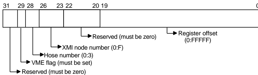
Figure 20–7 VMEbus Pseudo CSR Address
