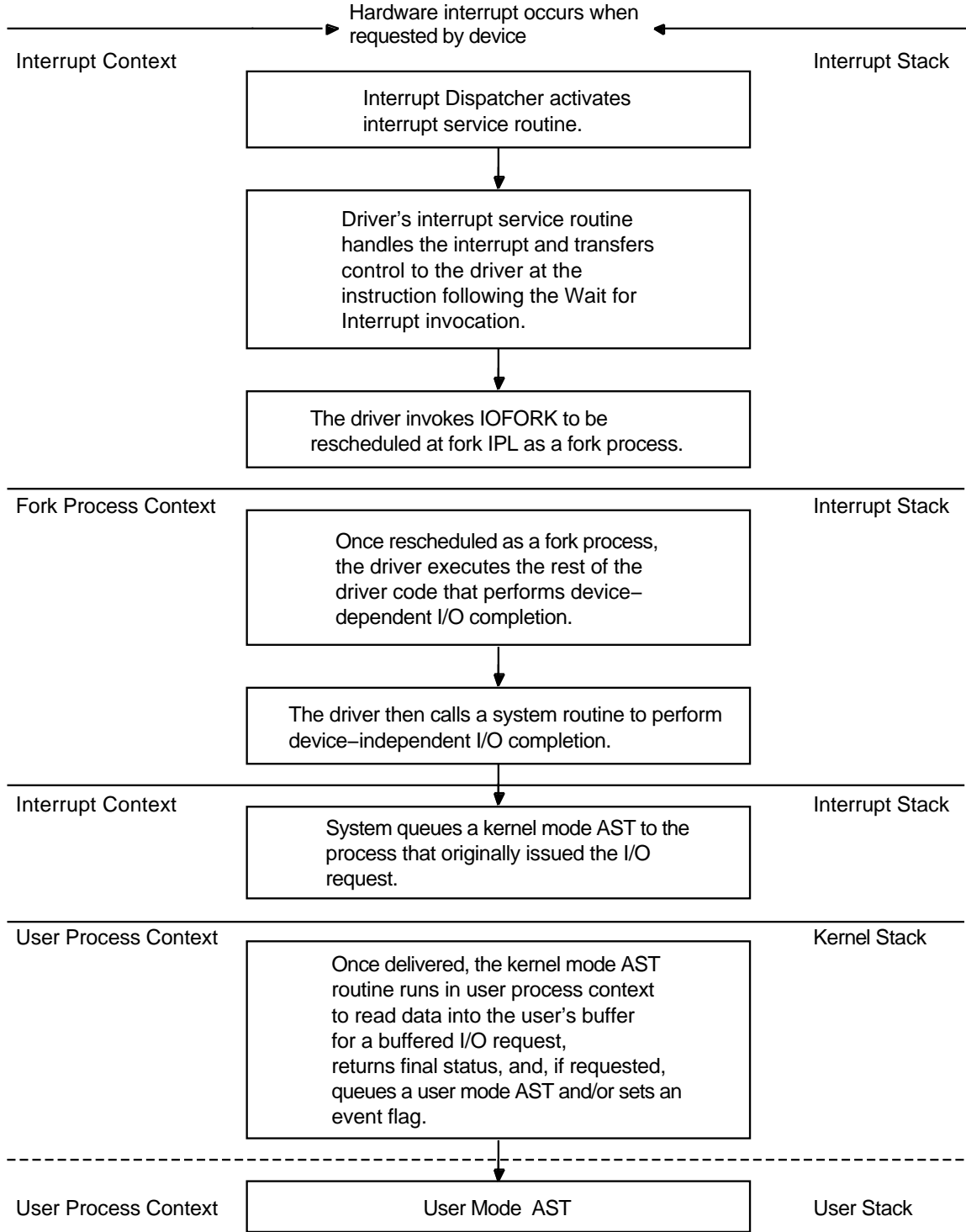
Figure 4-1 (Cont.) Sequence of Driver Execution
