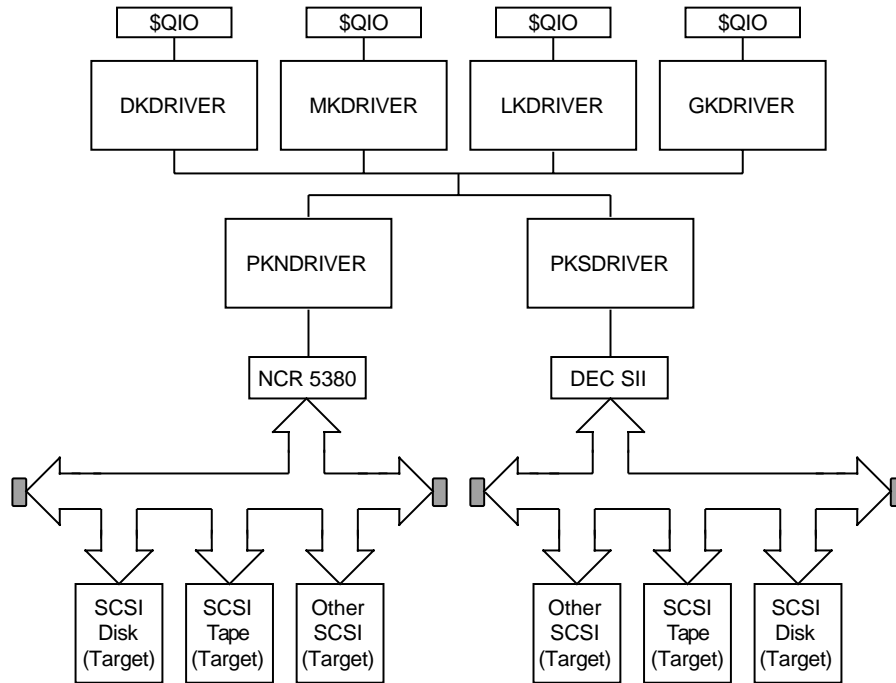
Figure 17-2 SCSI Port Driver Configuration
