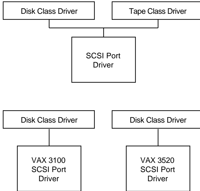
Figure 17–3 SCSI Class Driver Configuration
