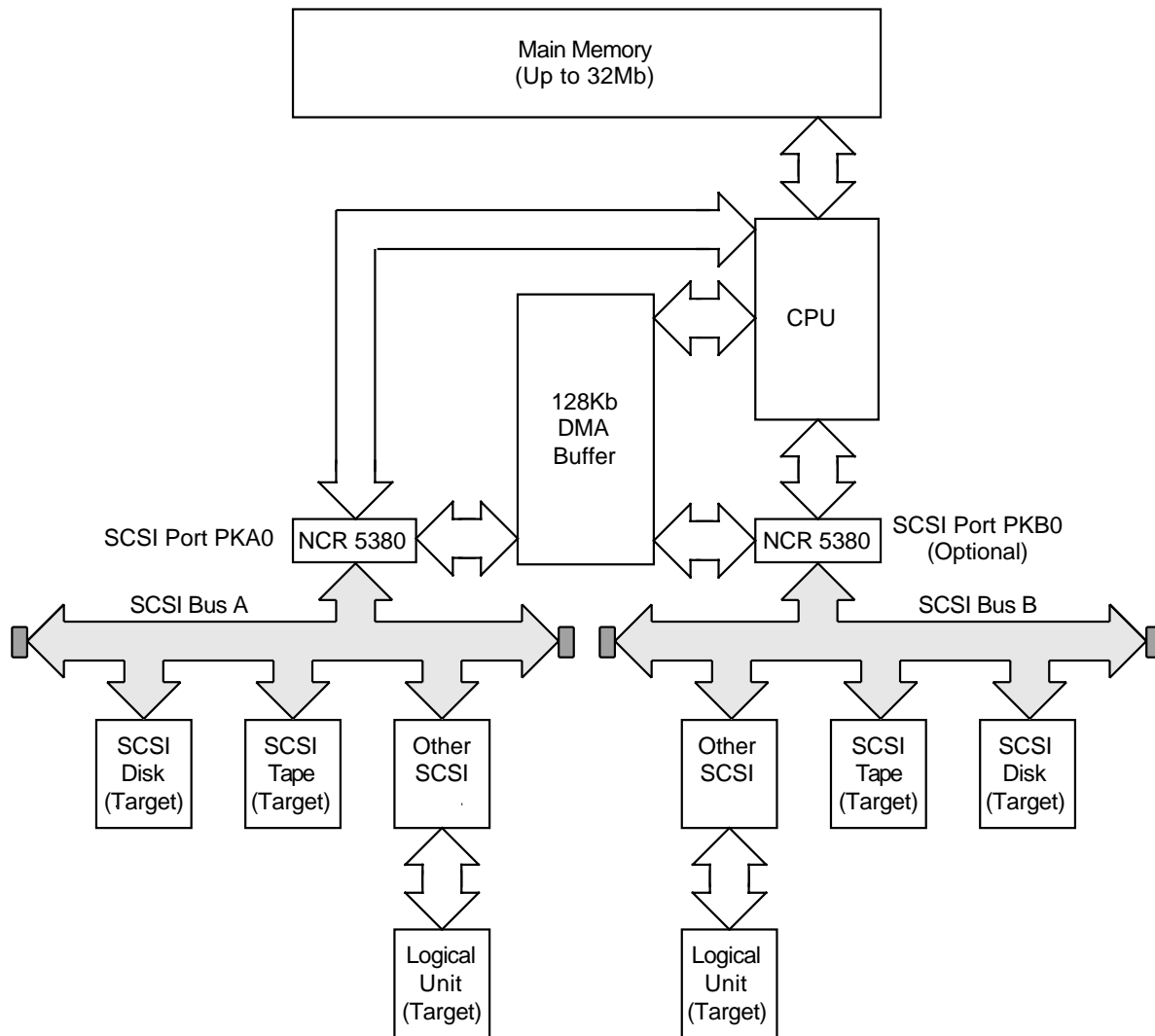
Figure 1–9 MicroVAX/VAXstation 3100 System Architecture
