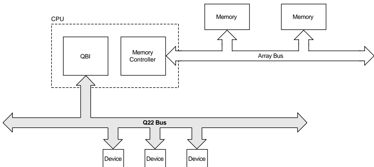
Figure 1-8 Q22-bus Based Systems
