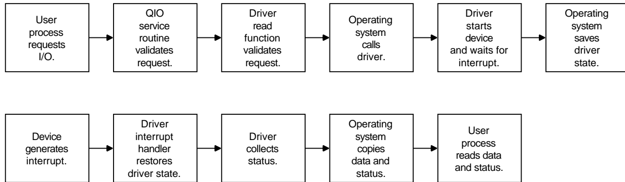
Figure 1–11 Example of I/O Request Processing
