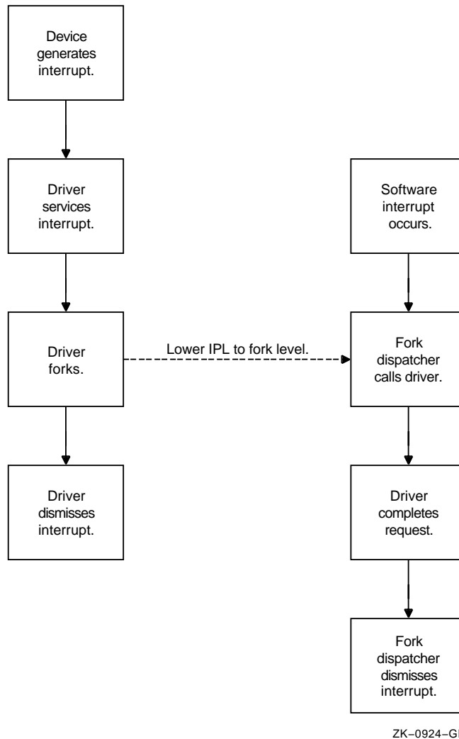
Figure 4–8 Reactivation of a Driver Fork Process
