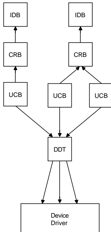
Figure 4-4 I/O Database for Two Controllers
