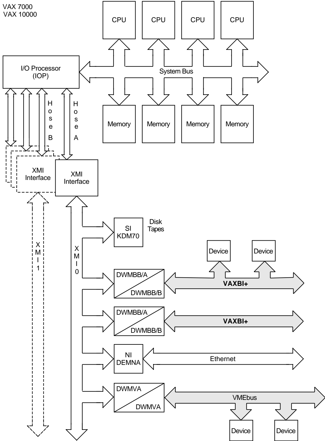
Figure 1-7 VAX 7000 Series and VAX 10000 Series System Architecture
