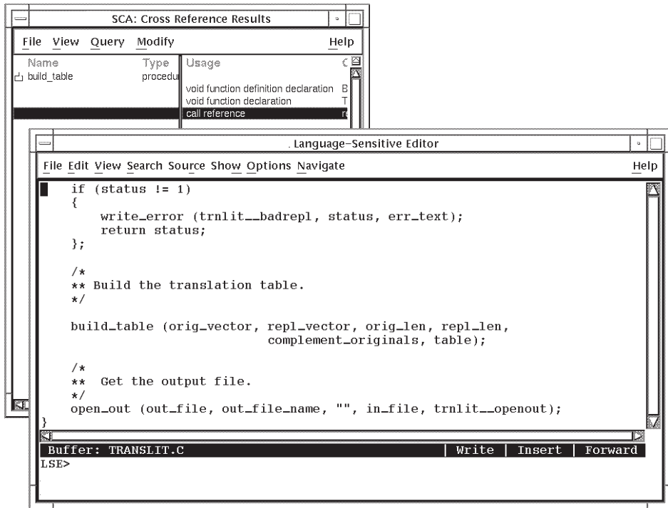
Figure 4-4 Go-To-Source Feature
