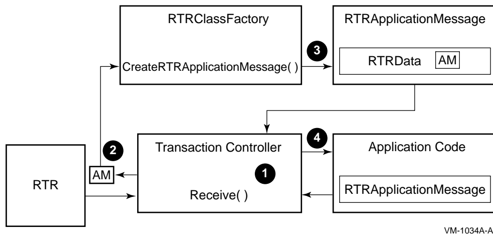
Figure 1–6 Receiving an Application Message
