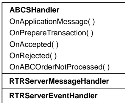
Figure 2–5 Sample Server-Handler-Derived Class
