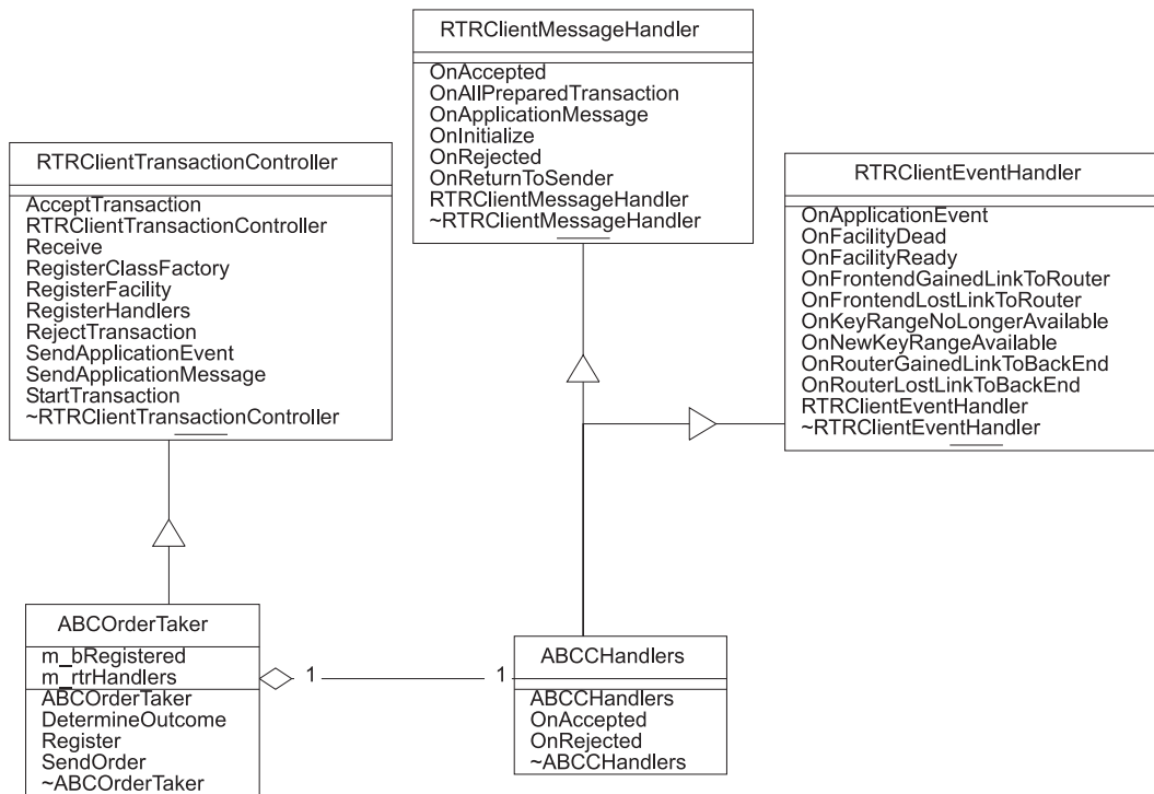
Figure B-3 Application Client Transaction Object Classes
