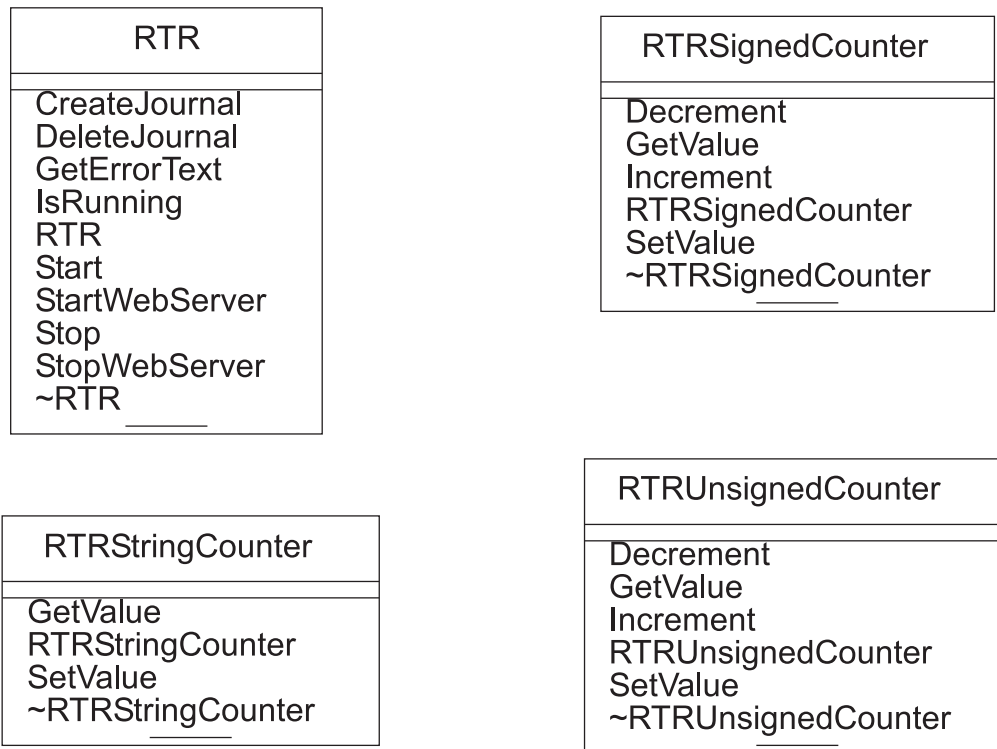
Figure A-4 Management Setup and Diagnostic Classes
