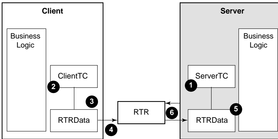
Figure 1–5 Client/Server Interaction
