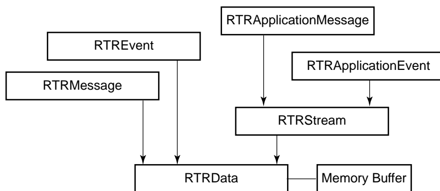
Figure 1–3 Data Classes
