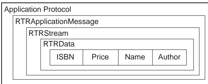
Figure 1–4 RTRData Encapsulation
