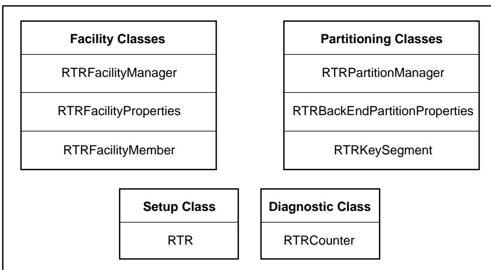
Figure 1–10 Management Classes
