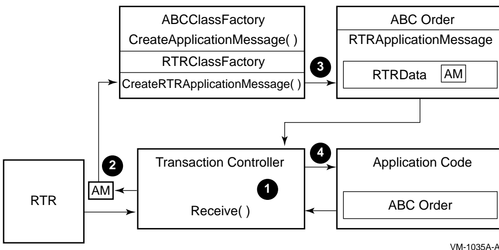
Figure 1–7 Receiving a User-Defined Application Message
