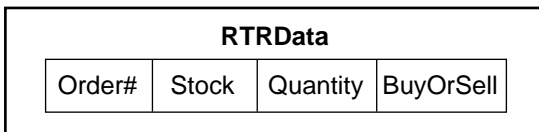
Figure 1–16 The Protocol Manager Object
