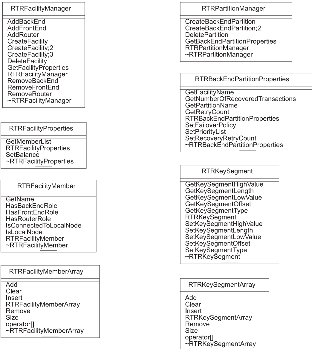
Figure A-3 Management Facility and Partition Classes
