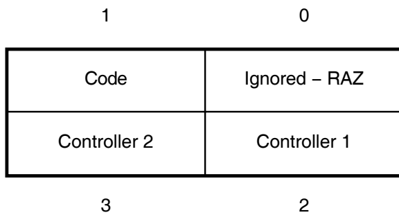
Figure F-1 Format of Quadword Buffer
