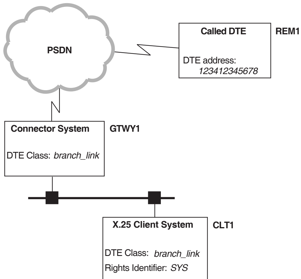
Figure 3–6 Example Outgoing Call from an X.25 Client System
