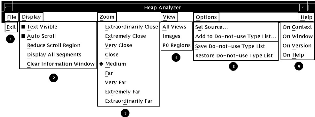
Figure 12–2 Heap Analyzer Pull-Down Menus
