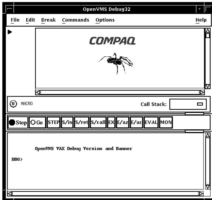
Figure 9–1 Debugger at Startup
