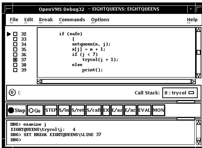
Figure 10–4 Setting a Breakpoint on a Source Line
