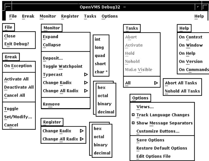
Figure 8–8 Menus on Optional Views Window
