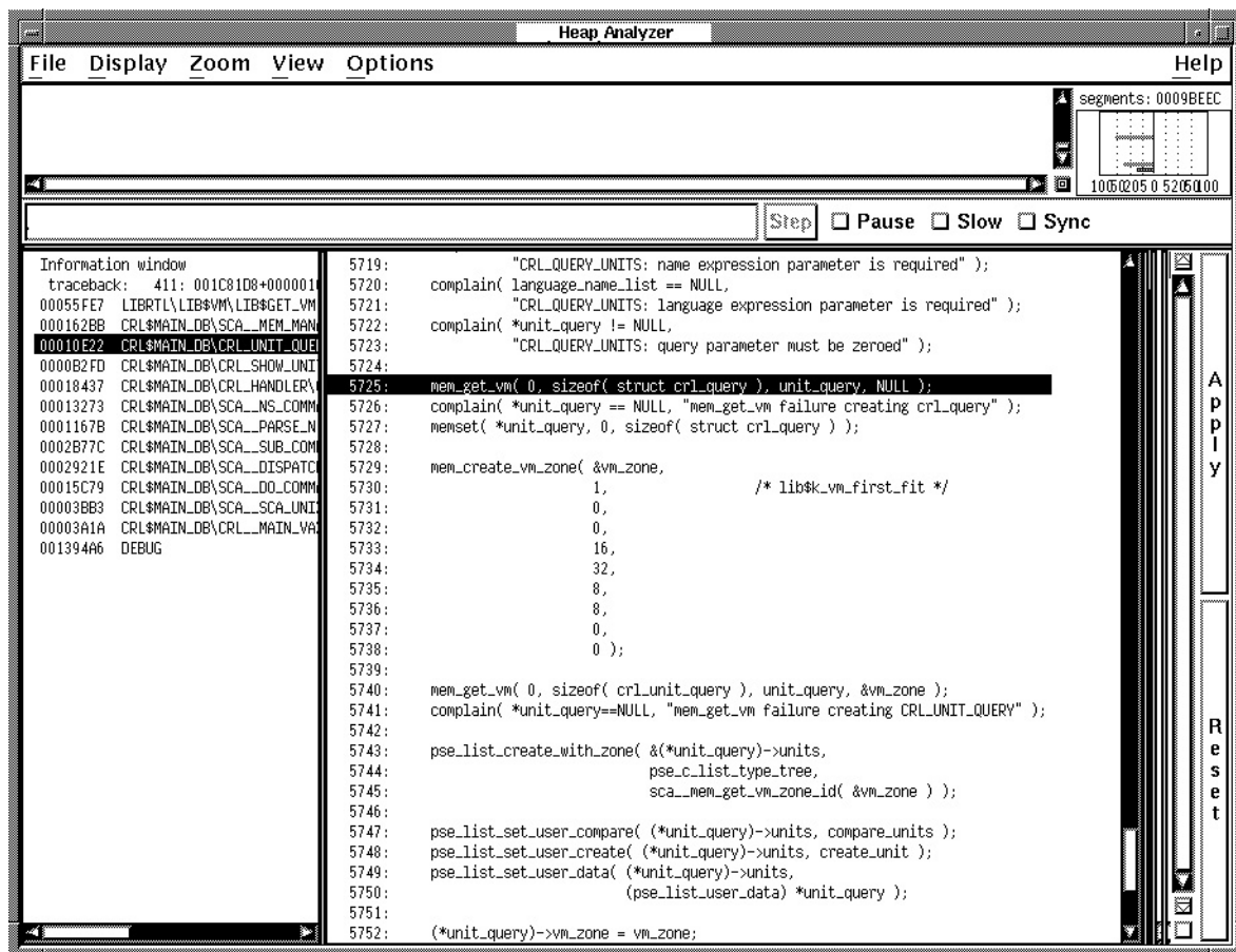
Figure 12–15 Review of Source Code Shows Double Allocation
