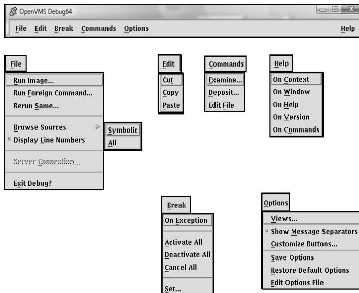
Figure 8–2 Menus on Main Window
