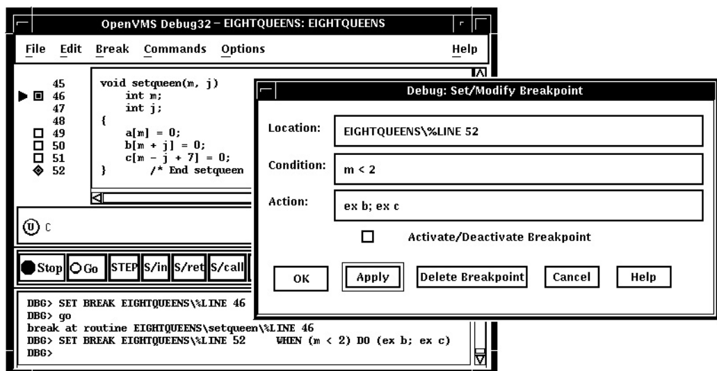
Figure 10–7 Setting an Action Breakpoint
