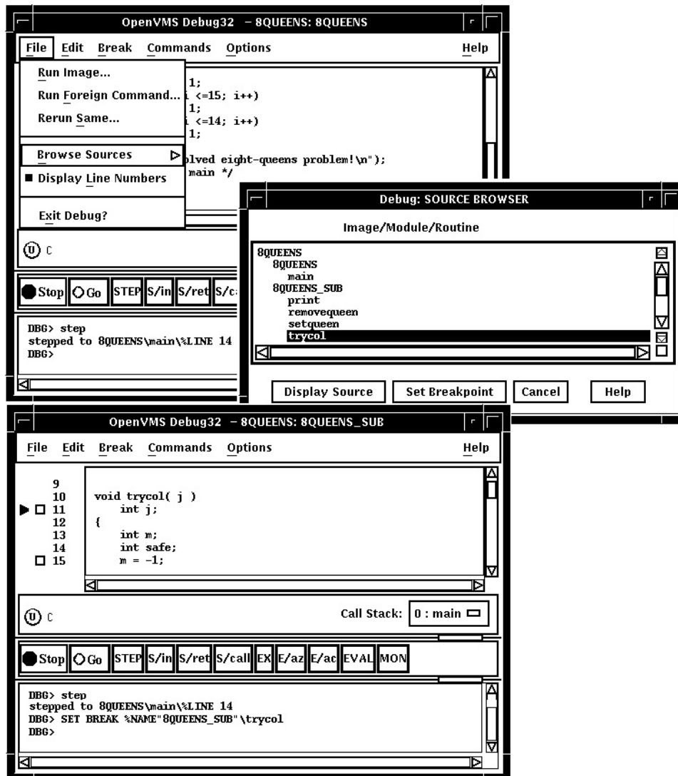
Figure 10–5 Setting a Breakpoint on a Routine
