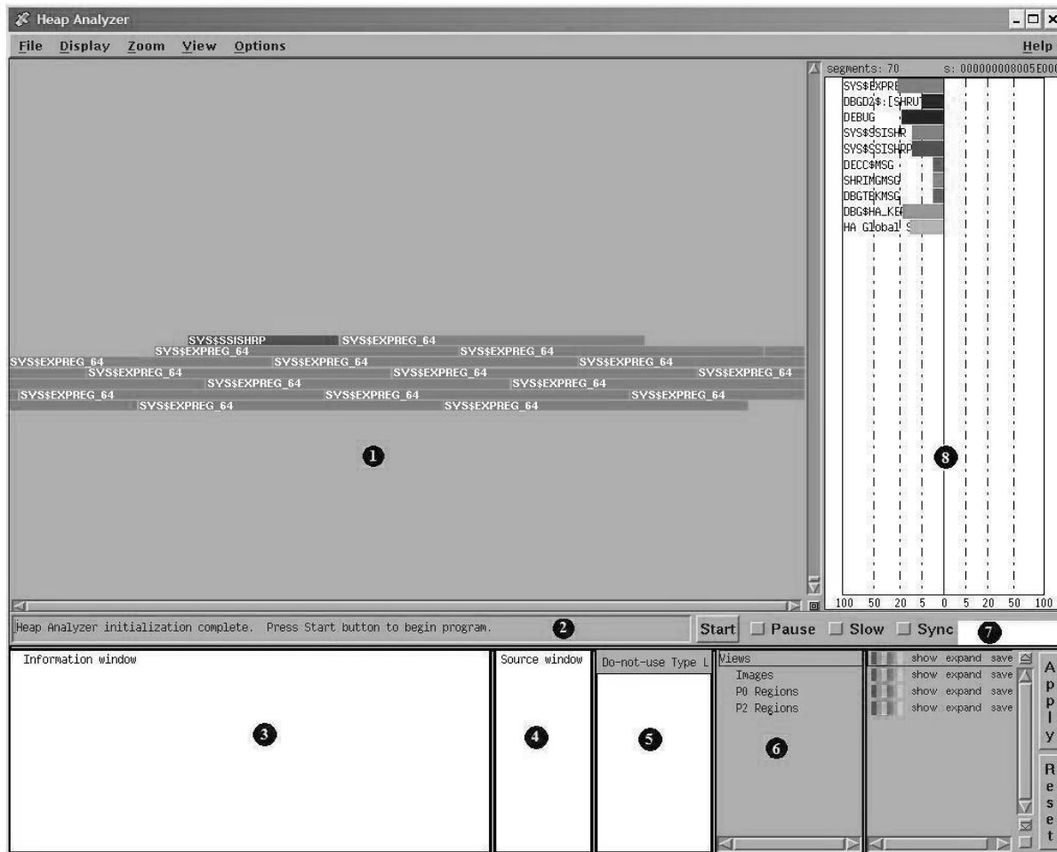
Figure 12–1 Heap Analyzer Windows
