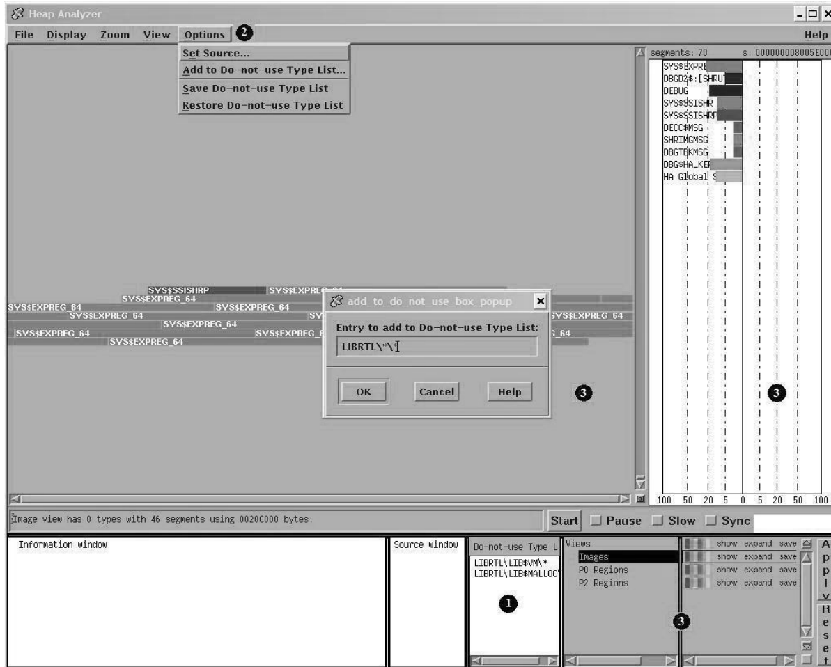
Figure 12–9 Heap Analyzer Do-Not-Use Type List
