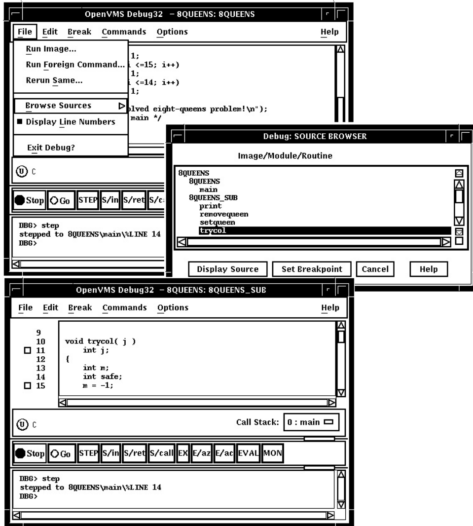
Figure 10–2 Displaying Source Code of Another Routine
