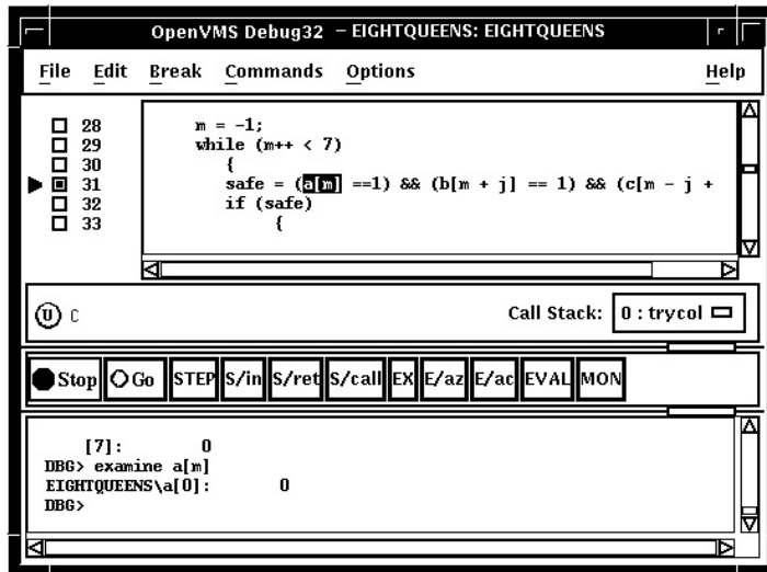
Figure 10–10 Displaying the Value of an Array Element
