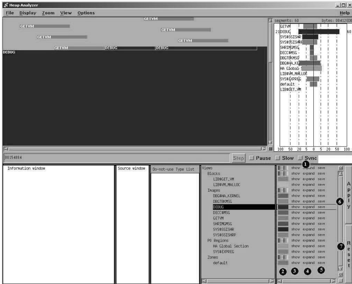
Figure 12–11 Heap Analyzer Views-and-Types Display Options
