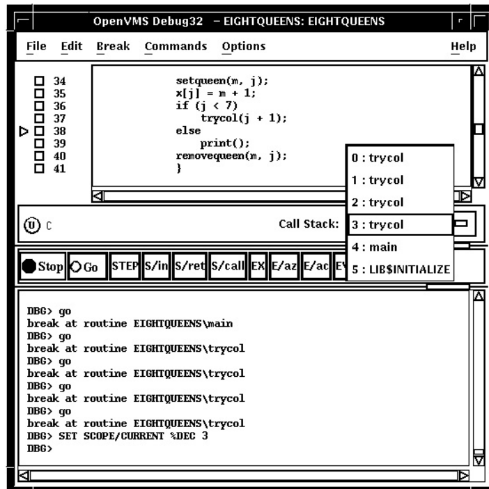
Figure 10–19 Current Scope Set to a Calling Routine
