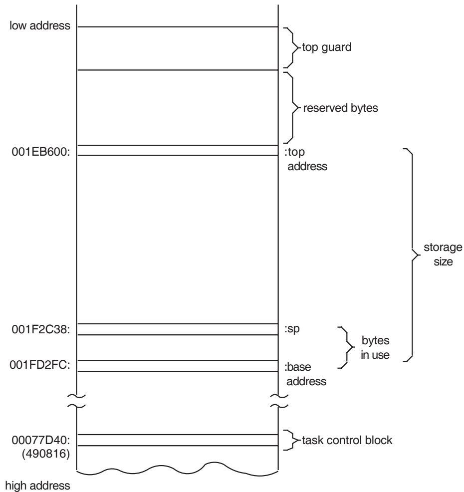
Figure 16–1 Diagram of a Task Stack
