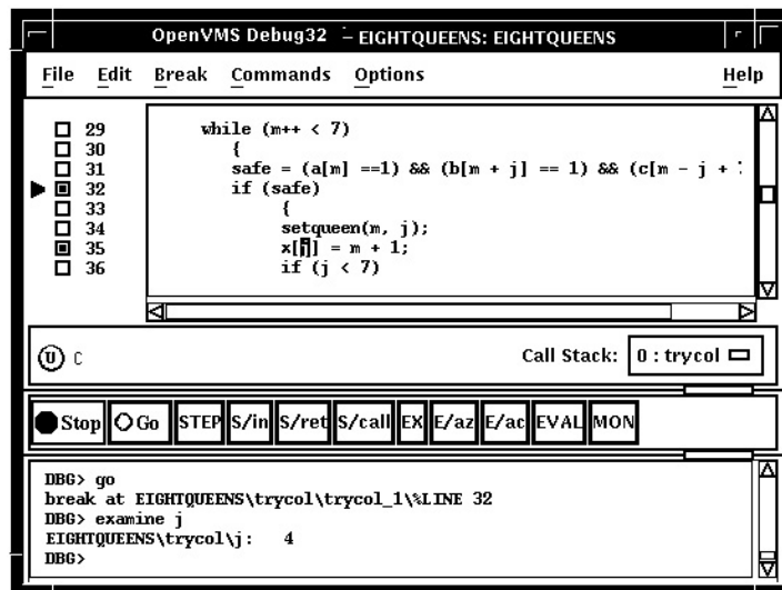
Figure 10–8 Displaying the Value of an Integer Variable
