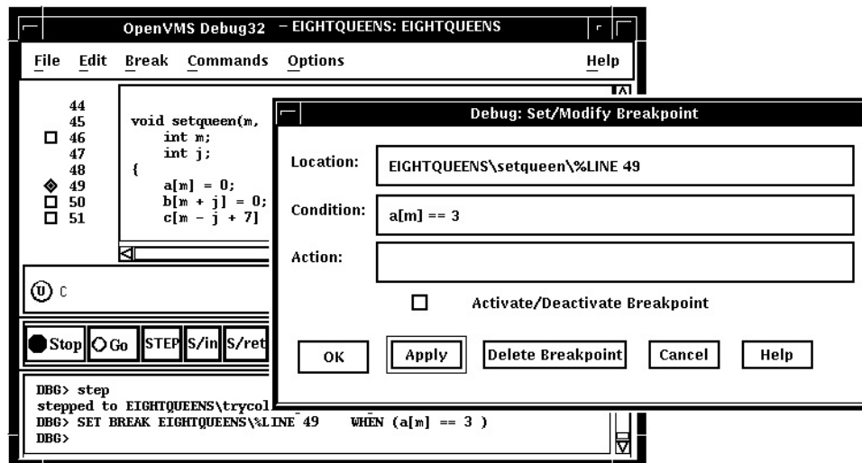
Figure 10–6 Setting a Conditional Breakpoint
