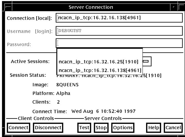
Figure 9–8 Active Sessions List
