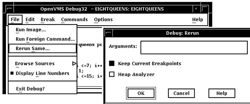
Figure 9–5 Rerunning the Same Program
