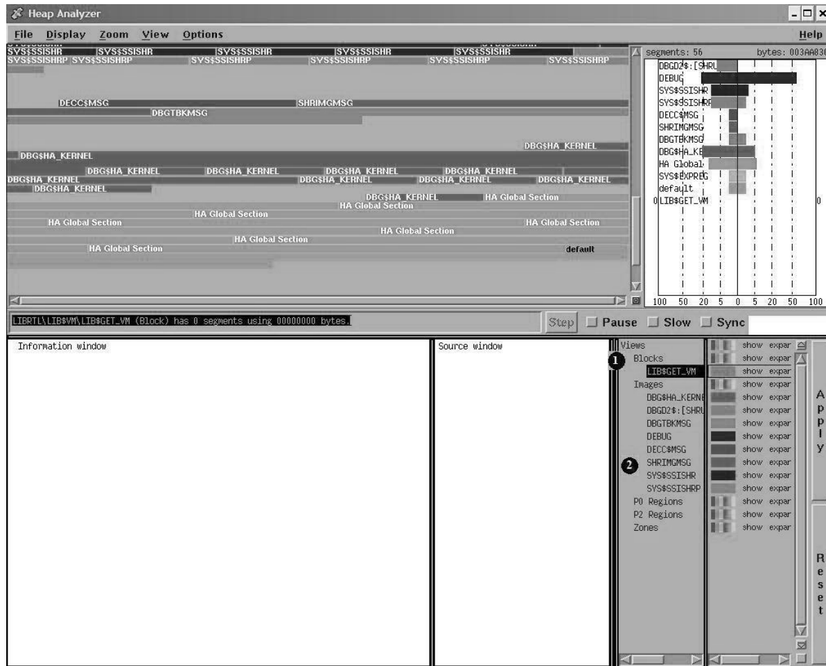
Figure 12–10 Heap Analyzer Views-and-Types Hierarchy
