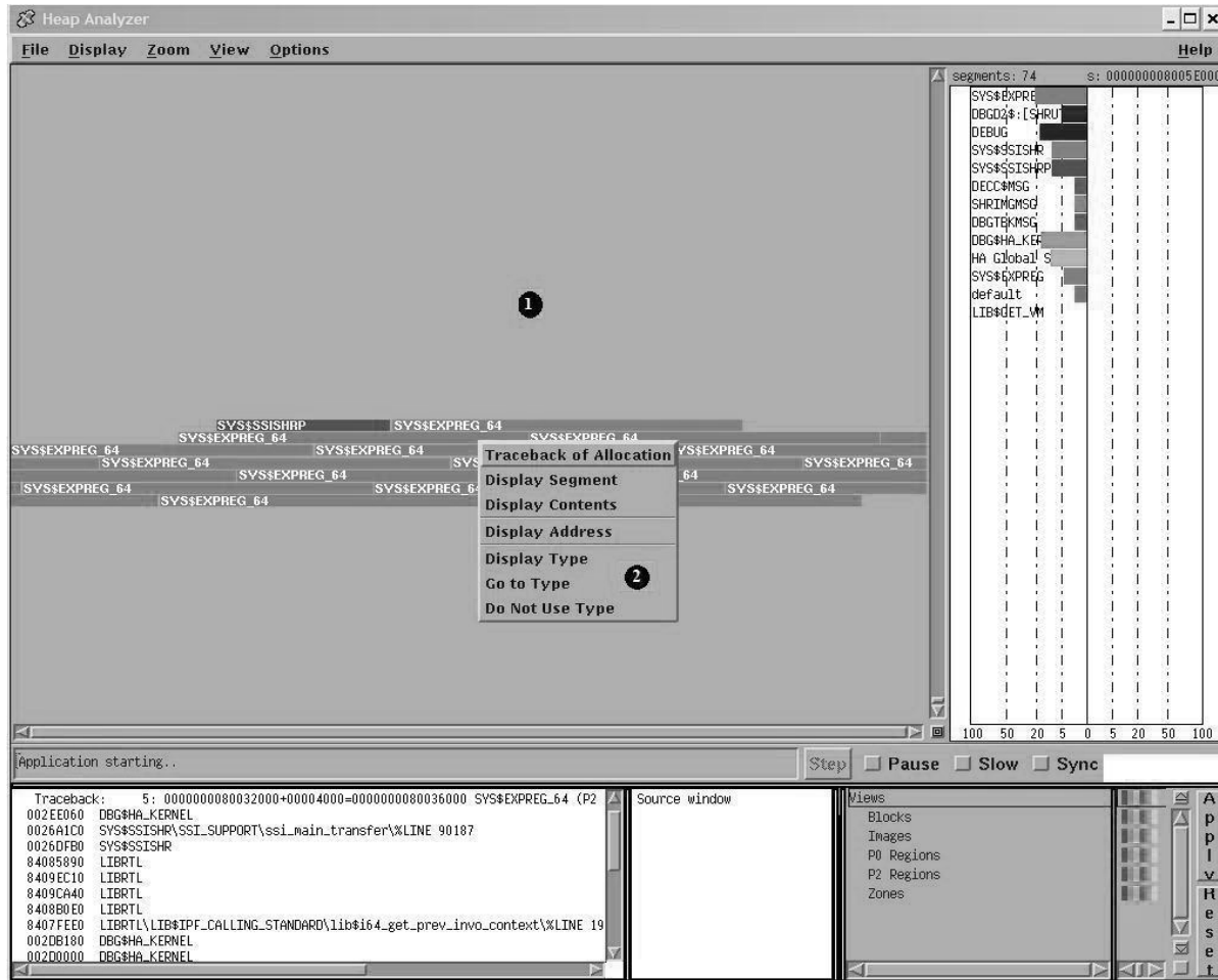
Figure 12–6 Heap Analyzer Memory Map Context-Sensitive Pop-Up Menu
