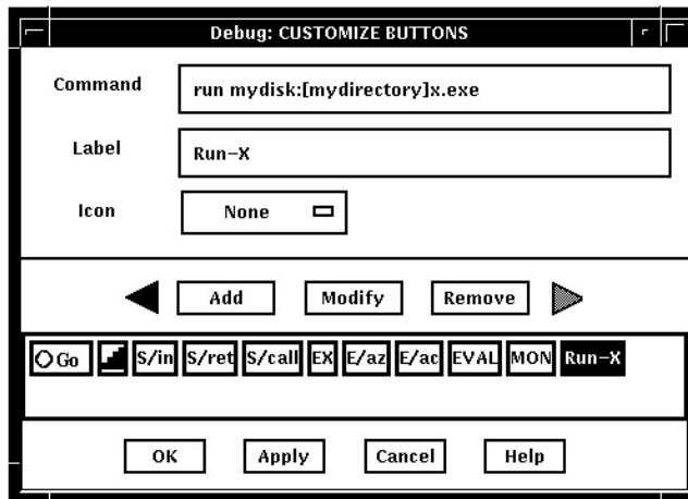
Figure 10–24 Adding a Button
