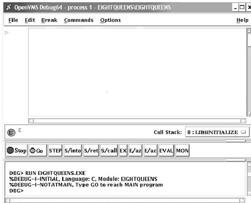
Figure 9-4 Source Display at Startup
