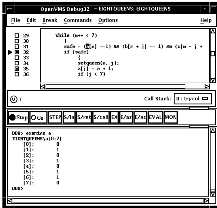
Figure 10–10 Displaying the Value of an Array Element
