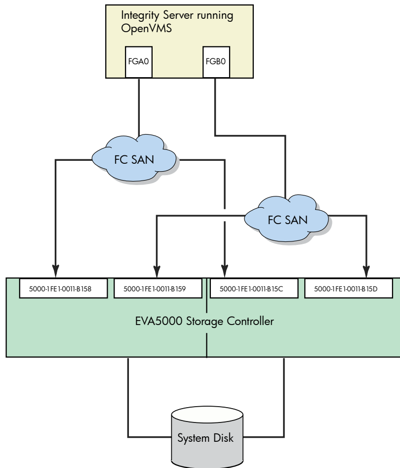
Figure D-1 Fibre Channel Host and SAN Storage Controller Configuration
